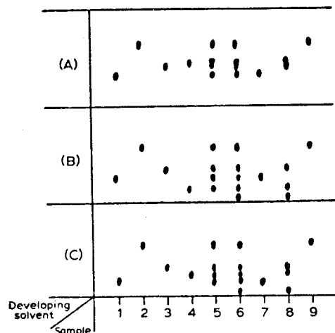
Fig. 1. Thin-layer chromatograms of clavine and lysergic acid alkaloids on Silica Gel G. Developing solvents: (A) acetone-piperidine (9:1); (B) chloroform-methanol (4:1); (C) acetone-ethyl acetate-dimethylformamide (5:5:1). Detection: Observation under UV light and spraying with Van Urk reagent. Samples: 1 = lysergic acid amide; 2 = isolysergic acid amide; 3 = lysergol; 4 = elymoclavine; 5 = 1 + 2 + 3 + 4; 6 = extract from Heavenly Blue seeds; 7 = fraction C obtained by column chromatography; 8 = fraction D obtained by column chromatography; 9 = fraction E obtained by column chromatography.
