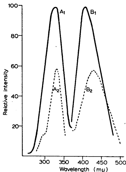
Fig. 1. Fluorescence excitation and emission spectra for LSD and quinine on a thin-layer chromatogram. Mixture containing 2.0 \mu g of LSD and 0.5 \mu g of quinine were spotted on the thin-layer plate, followed by development in the solvent system (A), MeOH-CHCl 3 - n -hexane (1:4:2). (A 1 ) Fluorescence excitation spectrum for LSD by setting emission at 410 m \mu ; (B 1 ) fluorescence emission spectrum for LSD by setting excitation at 330 m \mu ; (A 2 ) fluorescence excitation spectrum for quinine by setting emission at 436 m \mu ; (B 2 ) fluorescence emission spectrum for quinine by setting excitation at 336 m \mu .
