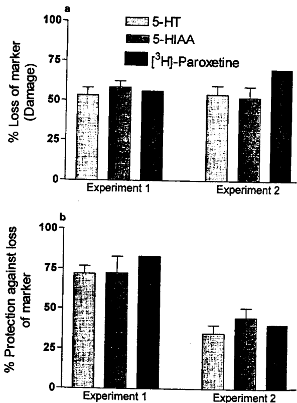
Figure 5 (a) The mean % loss of 5-HT and 5-HIAA in the 3 areas examined (± s.e.mean) and mean % loss of [3H]-paroxetine binding in the MDMA-treated group in the experiment presented in Figure 3 (Experiment 1) and the experiment shown in Figure 4 (Experiment 2). (b) The mean % protection against MDMA-induced loss of 5-HT and 5-HIAA and mean % loss of [3H]-paroxetine binding in the MDMA + clomethiazole treated group kept at normal ambient temperature and shown in Figure 3 (Experiment 1) and the group given MDMA + clomethiazole kept at high ambient temperature in the experiment illustrated in Figure 4 (Experiment 2).
