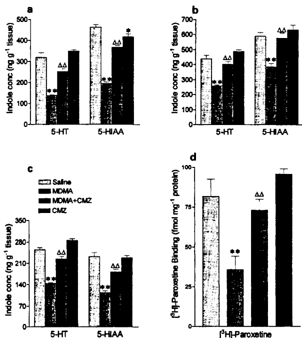
Figure 3 The indole concentrations in (a) hippocampus, (b) striatum, (c) cortex and (d) [3H]-paroxetine binding values in cortex 7 days following saline or clomethiazole (CMZ, 50 mg kg -1 ) 5 min before and 55 min after saline or MDMA (15 mg kg -1 ). Results shown as mean ± s.e.mean, n = 5. Different from saline-treated: * P < 0.05, ** P < 0.01; different from MDMA-treated: ΔΔ P < 0.01.
