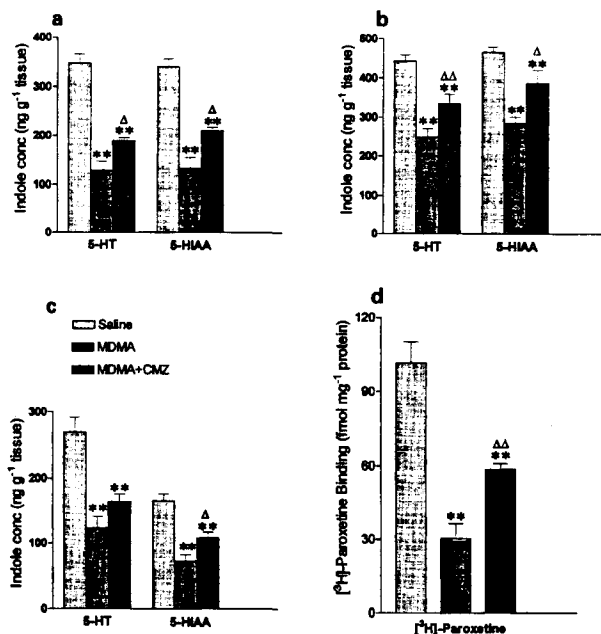
Figure 4 The indole concentrations in (a) hippocampus, (b) striatum, (c) cortex and (d) [3H]-paroxetine binding values in cortex 7 days following saline or clomethiazole (CMZ, 50 mg kg -1 ) 5 min before and 55 min after saline or MDMA (15 mg kg -1 ). The MDMA + clomethiazole rats were kept at high ambient temperature during the 5 h after the second CMZ injection. Results shown as mean ± s.e.mean, n = 4–5. Different from saline-treated: ** P < 0.01. Different from MDMA-treated: Δ P < 0.05, ΔΔ P < 0.01.
