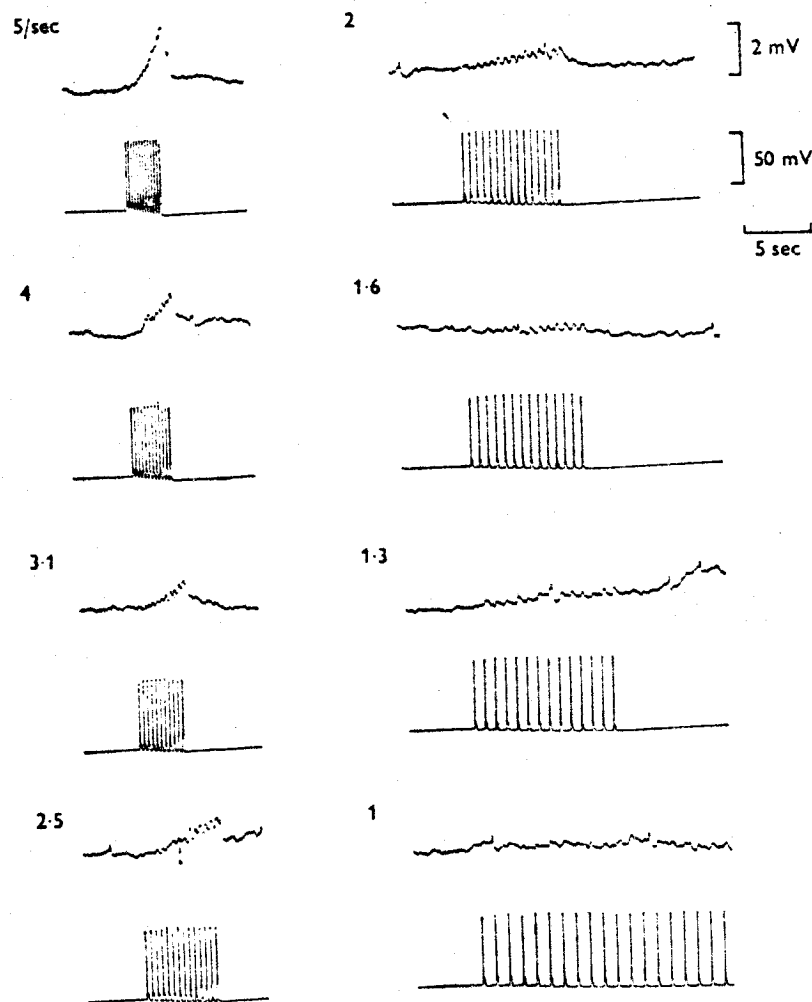
Fig. 5. Effect of frequency of giant serotonin cell action potentials on e.p.s.p. summation and facilitation in the middle cell. The middle cell was impaled with a KCl/Na 2 SO 4 double-barrelled electrode. Top trace in each pair is the middle cell membrane potential and the lower trace the giant serotonin cell membrane potential. The middle cell resting potential was –60 mV, but was artificially hyperpolarized to –100 mV during the experiment; the giant serotonin cell resting membrane potential was –50 mV. Summation of e.p.s.p.s occurred at frequencies of 2 Hz or above, whereas facilitation occurred at lower frequencies.
