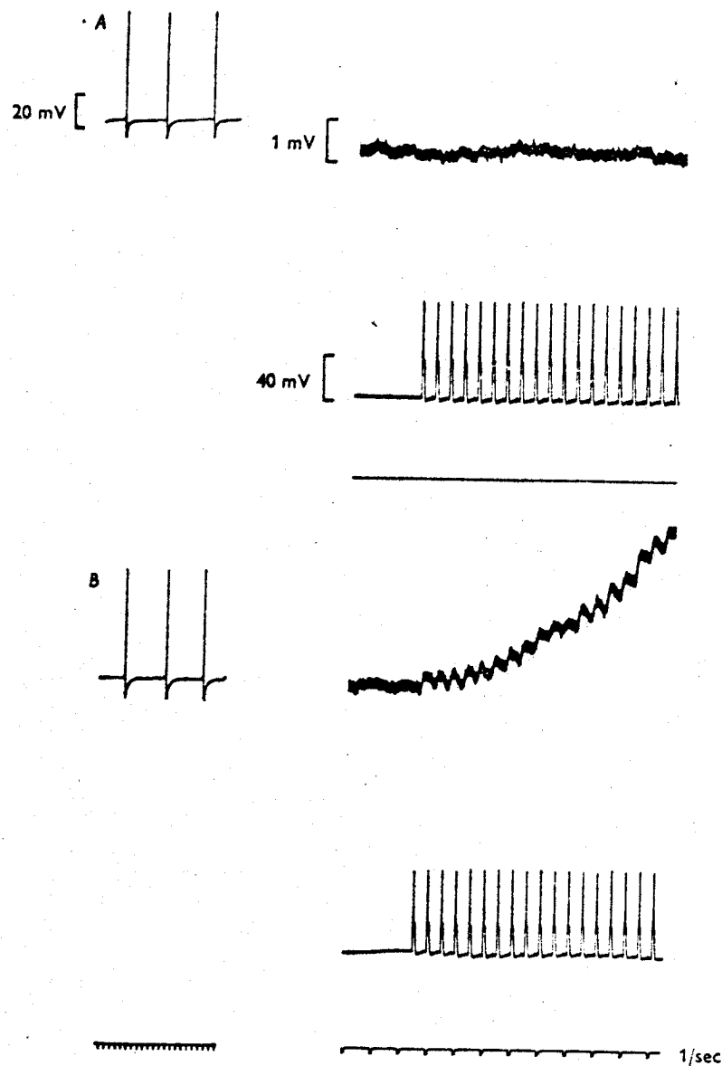
Fig. 16. Effect of low Na medium (12 mM-NaCl and 68 mM-LiCl) on the middle cell e.p.s.p.s. The middle cell was impaled with two separate KCl electrodes and hyperpolarized by 40 mV to -95 mV during periods of recording. Upper trace in each pair is the middle cell potential; lower trace is the giant serotonin cell potential. A , absence of middle response to giant cell stimulation after exposure to low Na medium for 30 min. B , e.p.s.p.s recorded after 12 min exposure to normal medium. Note that the height of the middle cell action potential (shown on the left) was the same in low Na medium as in the normal medium.
