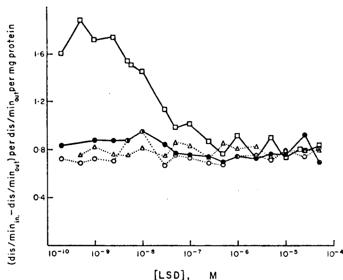
FIG. 1. Binding of LSD to synaptosomes (▲) and synaptic membranes (□) from cerebral cortical gray matter, and myelin (○), synaptosomes (●), and mitochondria (△) from whole brain exclusive of cerebral cortical gray matter. For multiple binding sites:
