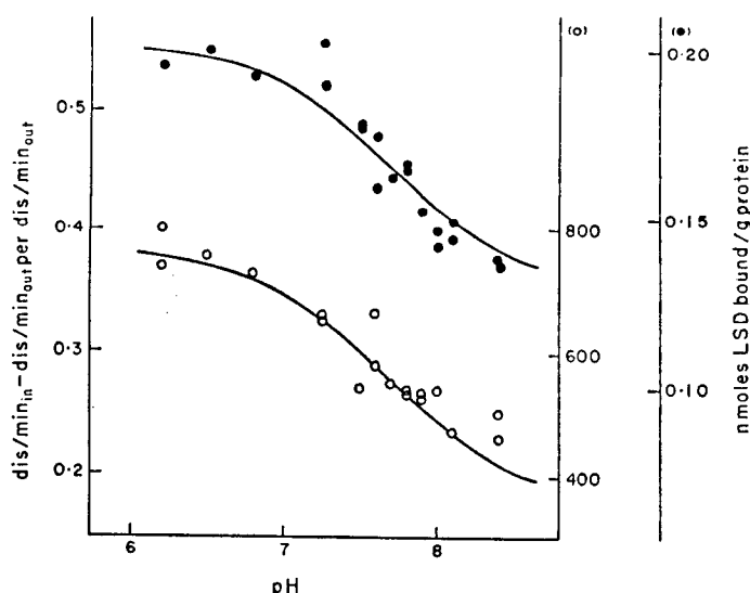
FIG. 4. Binding of 5 \times 10^{-9} M LSD (top) and 2 \times 10^{-5} M LSD (bottom) to synaptosomes at various pH values. Points are experimental data, and the curves are theoretical curves for proton dissociation, pK = 7.70 (top), pK = 7.65 (bottom). LSD has a pK value of 7.72. 12
