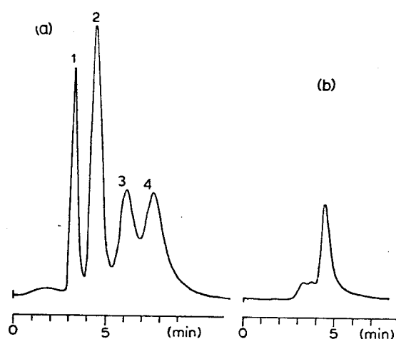
Fig. 2. LC separation of LSD on a 1.2-m column containing Corasil C 18 with 6:4 methanol-0.1% ammonium carbonate solution as solvent. (a) A synthetic mixture: 1=ergometrine maleate, 2=LSD, 3=iso-LSD, 4=ergotamine tartrate. (b) A tablet extract.
