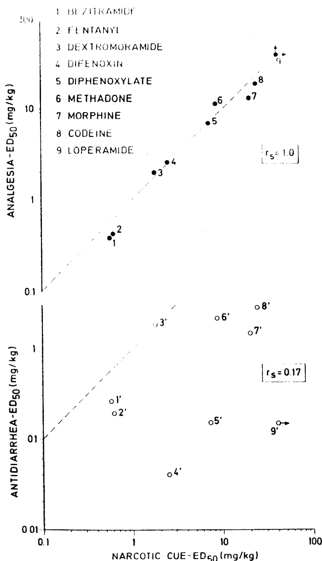
FIG. 7. Graphical representation of the differential quantitative relations between narcotic cuing activity on the one hand, and analgesic and constipating activity on the other. Log-log plot of ED_{50} values for stimulus generalization with fentanyl (abscissa), for analgesia (upper ordinate), and for constipation (lower ordinate).
