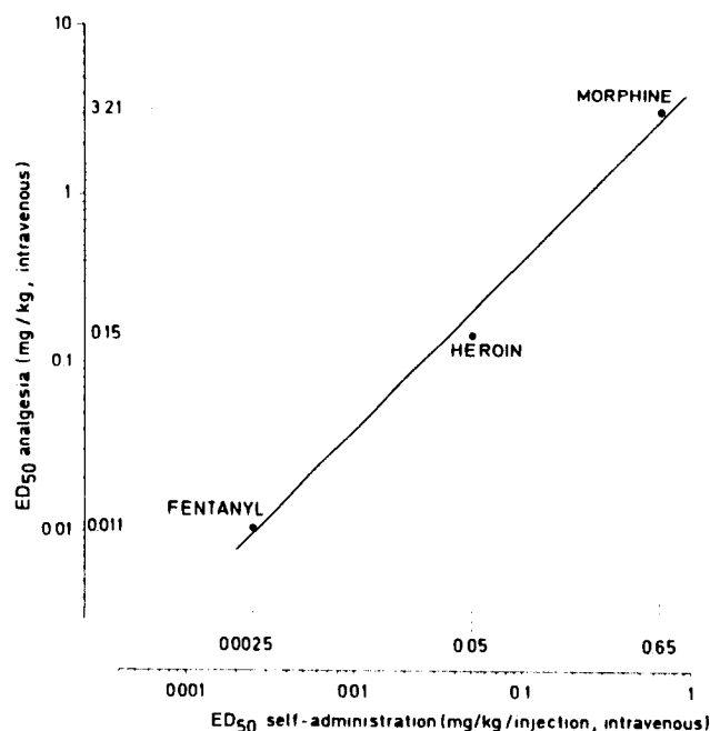
FIG. 9. Analgesic and primary reinforcing potency of intravenously administered fentanyl, heroin and morphine in rats. Log-log plot of ED_{50} for self-administration (abscissa) and analgesia (ordinate). The self-administration data are adopted from Van Ree, et al. [152]; the analgesia data are courtesy of Dr. C. J. E. Niemegeers (unpublished).
