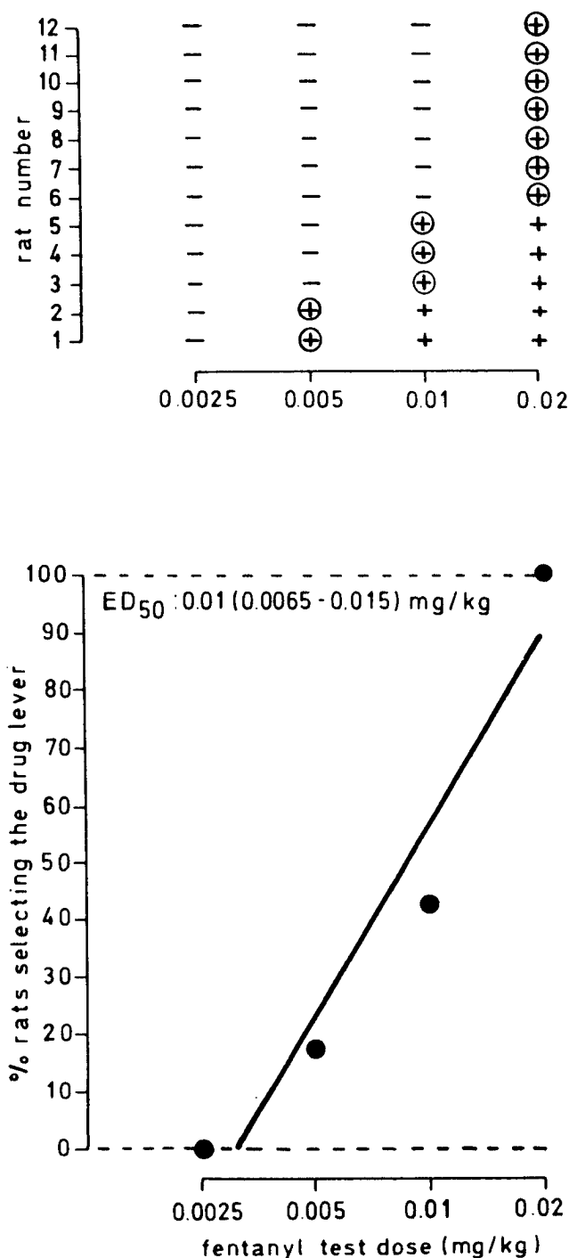
FIG. 3. Stimulus generalization of lower fentanyl doses with the training dose in rats ( n=12 ) trained to discriminate 0.04 mg/kg fentanyl from saline. In the top section, lever selection data are presented for each rat individually (- refers to Saline Lever; + refers to Drug Lever); the individual lowest effective, or threshold, dose is encircled. The bottom section represents the same data by a linear regression line on a log-linear plot.
