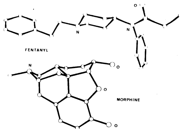
FIG. 1. Three-dimensional representation (J.P. Tollenaere and H. Moereels, unpublished data) of fentanyl and morphine obtained by X-ray crystallographic techniques [73,95]. For the sake of clarity, hydrogen atoms and double bonds are not shown.
