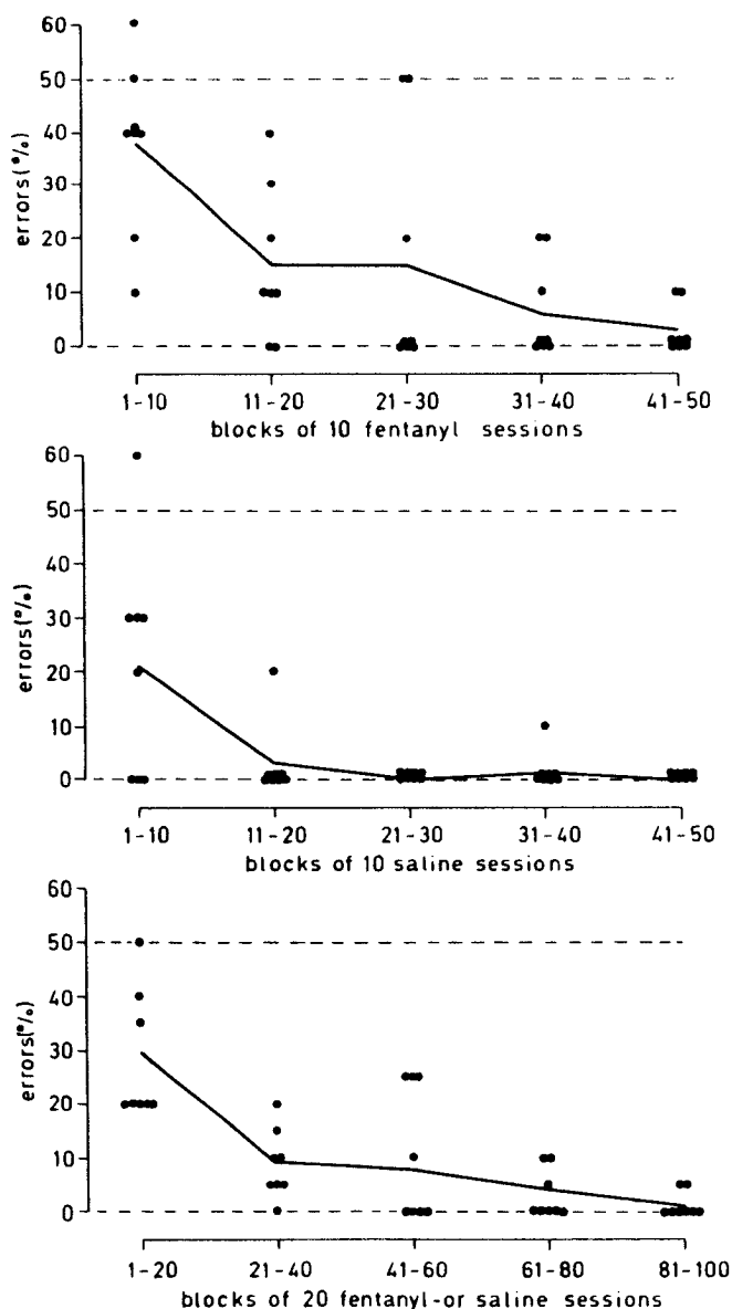
FIG. 2. Error rate as a function of training sessions in rats ( n=8 ) trained to select the correct out of two levers with 0.04 mg/kg fentanyl and saline serving as a pair of discriminative stimuli. Each point represents 10 (top and middle sections) or 20 (bottom section) observations in one animal. The solid lines connect points of overall error rate (all rats combined).
