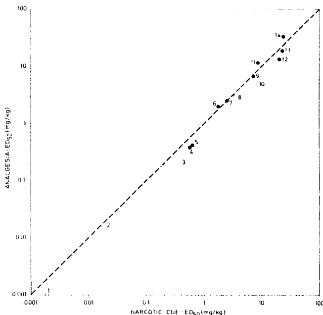
FIG. 5. Narcotic cueing and analgesic activity of narcotic analgesic drugs; log-log plot of ED_{50} values for stimulus generalization with fentanyl (abscissa) and for analgesia (ordinate). The numbers refer to the serial numbers of drugs as indicated in Table 3.
