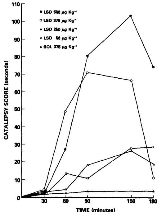
Fig. 1. Time course of the dose-dependent cataleptic response evoked by LSD. Various doses of LSD (50-500 µg kg -1 ) and a 375 µg kg -1 dose of BOL were administered subcutaneously and the intensity of catalepsy (in sec) was recorded at 30, 60, 90, 150 and 180 min respectively, following LSD administration, as described previously. Each point represents the mean cataleptic score of six animals.
