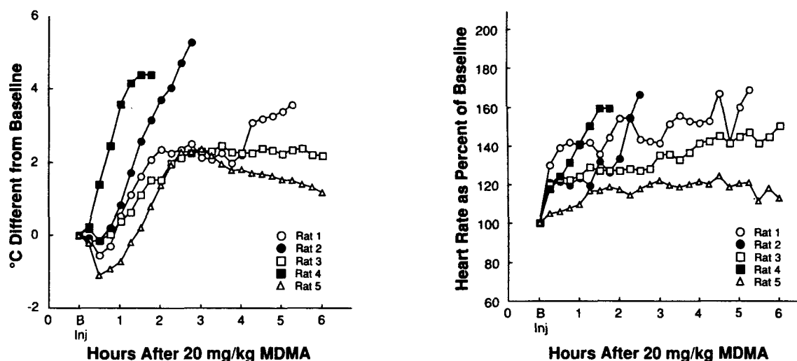
FIG. 7. Time-course of change in T_{core} and % change in HR of five rats injected with 20 mg/kg (SC) and maintained at a T_a of 25°C. Rats were permitted to acclimate to the experimental conditions for 90 min prior to MDMA administration. Rats 1, 2, and 4 died following collection of the last plotted data points.
