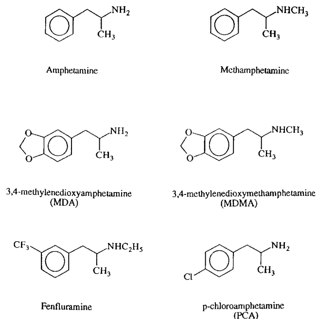
Fig. 1 Structure of MDMA and other substituted amphetamines
