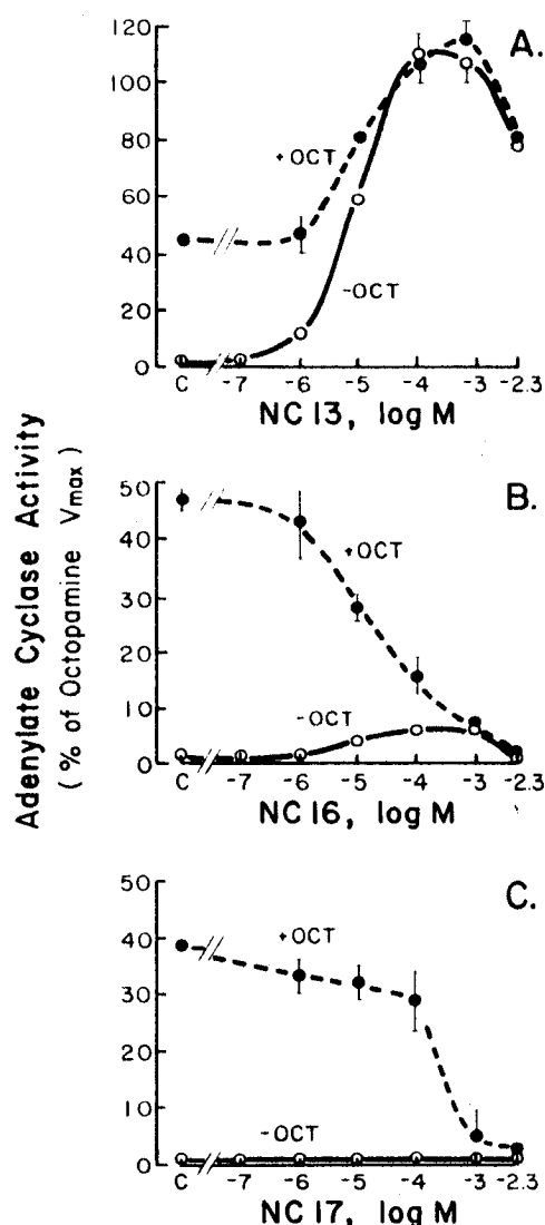
FIG. 4. Effects of PII derivatives on light organ adenylate cyclase activity, in the absence or presence of a fixed (10 \mu M) concentration of octopamine (OCT).
