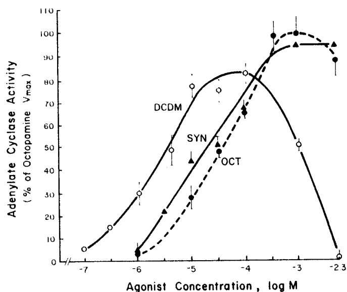
FIG. 2. Effects of the formamidine (DCDM) and the phenylethanolamine (SYN), compared with octopamine (OCT), on light organ adenylate cyclase activity.
