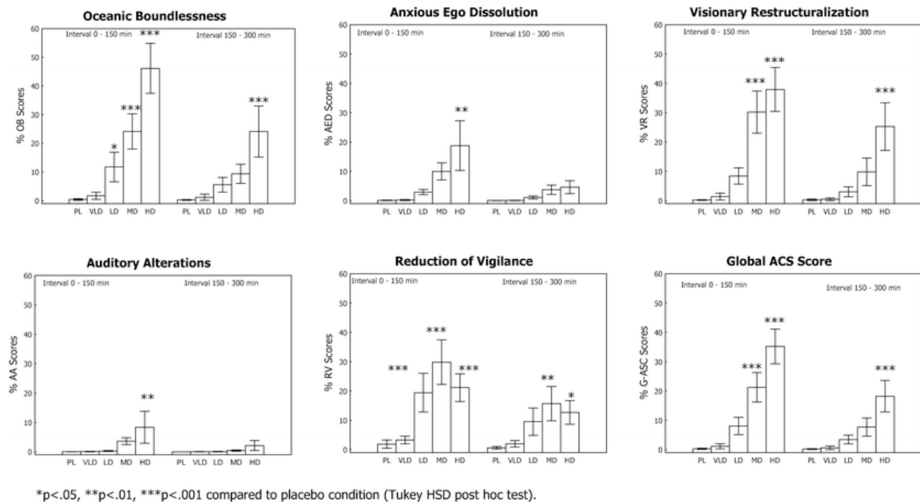
Fig. 1 Subjective effects of psilocybin. Percentage scores from the altered states of consciousness rating scale 5D-ASC (mean±SEM, n=8 ). Scores indicate percentage of theoretical scale maxima
