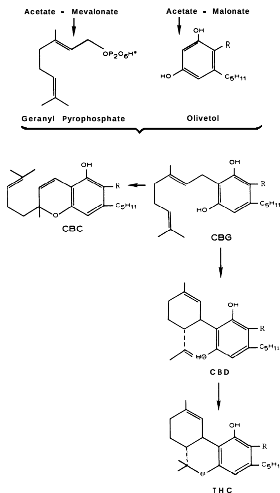
FIG. 1. -Proposed cannabinoid biosynthetic pathway (MECHOULAM 1970; C. E. TURNER et al. 1980). The presumed precursors, geranyl pyrophosphate and olivetol, are interpreted to give rise to CBG from which CBD, THC, and CBC are derived. These compounds occur principally as the carboxylated form ( R = \text{COOH} ) in the plant and are converted to the neutral form ( R = \text{H} ) on heating or drying of plant material.
