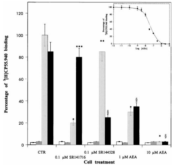
FIG. 2. Analysis of functional cannabinoid receptors in different cell lines. Binding of the synthetic cannabinoid [ 3 H]CP55.940 (400 pM) to CHP100 (white bars), U937 (gray bars), C6 (light gray bars), and DAUDI (black bars) cells and displacement by 0.1 \mu M SR141716, 0.1 \mu M SR144528, or 1 \mu M AEA. Unspecific binding was measured in the presence of 10 \mu M AEA. Values were expressed as percentage of the maximum (100% = 1000 \pm 100 cpm). Inset, binding of [ 3 H]CP55.940 (400 pM) by rat brain membranes and displacement by various concentrations of AEA. Values were expressed as percentage of the maximum (100% = 1000 \pm 100 cpm). CTR, control. *, p < 0.01 compared with control C6 cells; **, p > 0.05 compared with control C6 cells; ***, p > 0.05 compared with control DAUDI cells; §, p < 0.01 compared with control DAUDI cells.
