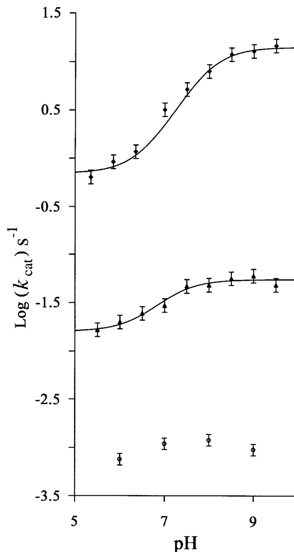
FIG. 4. pH versus k_{\text{cat}} profiles for oleamide hydrolysis by FAAH, the S217A mutant, and the S218A mutant. The pH dependences of k_{\text{cat}} for oleamide hydrolysis by FAAH (solid diamonds), the S218A mutant (solid triangles), and the S217A mutant (open circles) are shown. Curve fits were obtained by non-linear least squares regression and indicate a basic residue involved in catalysis with a pH of 7.9 (FAAH) or 7.1 (S218A). The lower activity limits for FAAH and the S218A mutants were 20- and 3.5-fold below the maximal activity, respectively. The S217A mutant exhibited less than a 30% change in activity between pH 6.0 and 9.0, and no ionizable residue pK_a values could be predicted from the profile.
