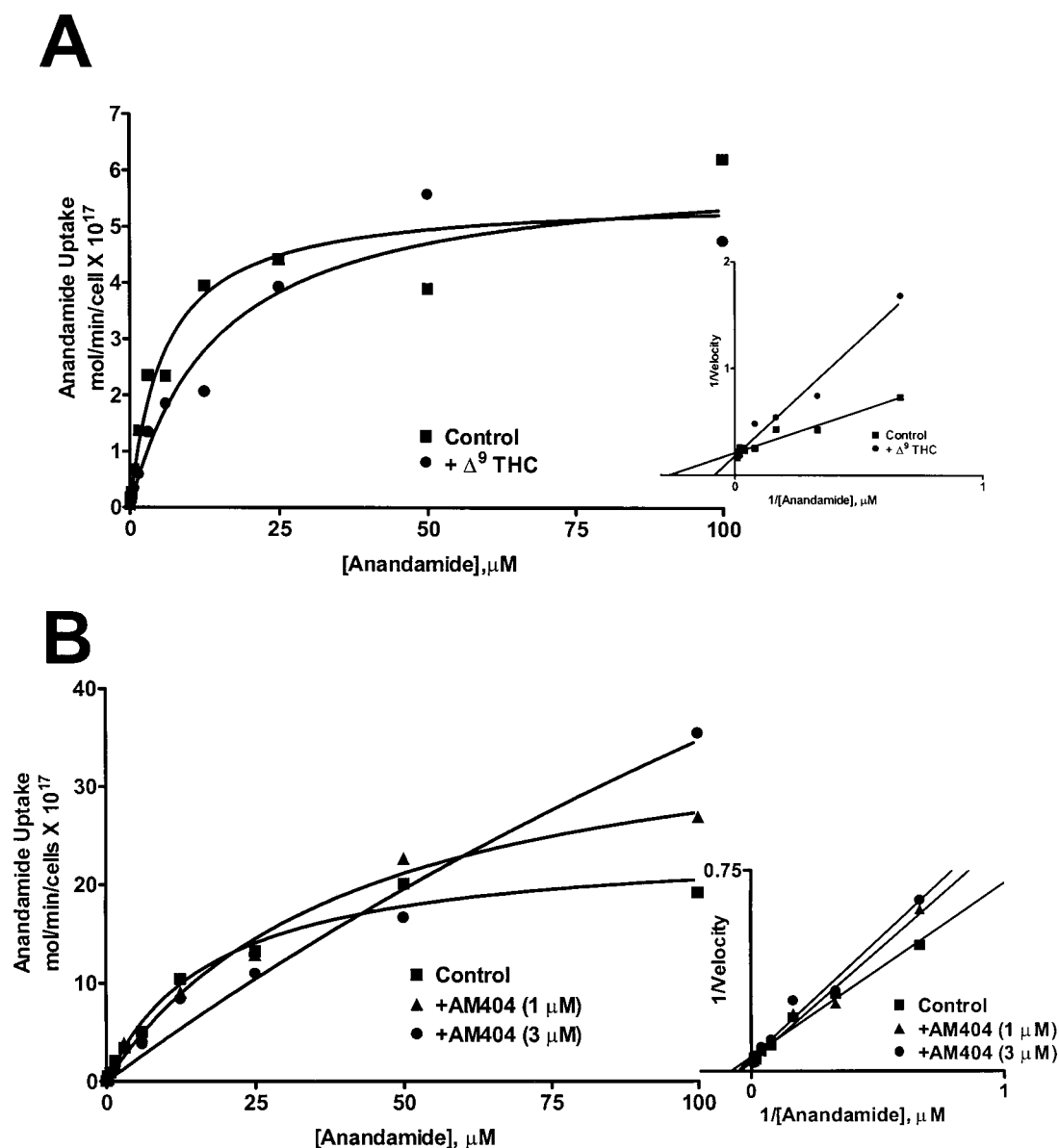
Fig. 4. Competitive inhibition of anandamide uptake by \Delta^9 -THC and AM404. RBL-2H3 cells were incubated with increasing concentrations of [ ^3\text{H} ]anandamide for 10 min at 37^\circ\text{C} in the presence or absence of 10 \mu\text{M} \Delta^9 -THC (A) or 1 or 3 \mu\text{M} AM404 (B). Nonspecific uptake was determined in the presence of 100 \mu\text{M} AM404 (A) or 100 \mu\text{M} ( R )-2-methanandamide (B). Data plotted are means of duplicate determinations and are representative of three separate experiments. Insets, Lineweaver-Burke plots of saturation curves shown above. Summary data for K_m and V_{\max} values were: A, control, 10.1 \pm 4.0 \mu\text{M} and 5.5 \pm 0.5 \times 10^{-17} mol/min/cell; +\Delta^9 -THC, 28.6 \pm 9.6 \mu\text{M} and 6.1 \pm 0.6 \times 10^{-17} mol/min/cell; B, control, 12.3 \pm 1.1 \mu\text{M} and 24.2 \pm 1.8 \times 10^{-17} mol/min/cell; +1 \mu\text{M} AM404, 40.3 \pm 17.0 \mu\text{M} and 32.2 \pm 5.9 \times 10^{-17} mol/min/cell; +3 \mu\text{M} AM404, 88.3 \pm 16.3 \mu\text{M} * and 57.7 \pm 3.0 \times 10^{-17} mol/min/cell*. * P < .05 compared with control value.
