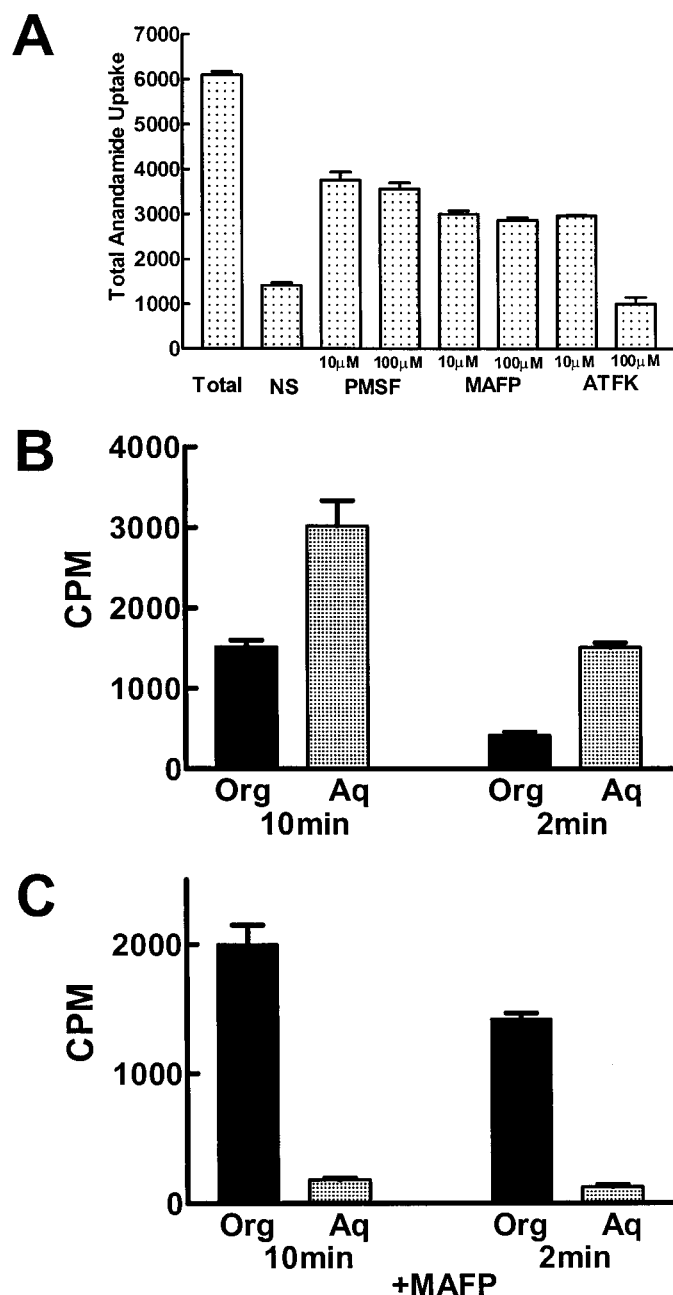
Fig. 3. Role of FAAH in anandamide uptake. A , sensitivity of anandamide uptake to FAAH inhibitors. Anandamide uptake was performed on RBL-2H3 cells as described in Experimental Procedures . Cells were treated with 10- and 100- \mu M concentrations of PMSF, MAFP, and ATFK 10 min before addition of 1 nM [ ^3 H]anandamide. Nonspecific (NS) uptake was determined in the presence of 100 \mu M AM404. Data were plotted as total anandamide uptake and are the means \pm S.E. of triplicate determinations and are representative of three separate experiments. B , metabolism of anandamide in RBL-2H3 cells. RBL-2H3 cells were incubated with 5 nM anandamide[ethanolamine 1- ^3 H] for indicated times, and extent of degradation by FAAH was determined as described in Experimental Procedures . Org = cpm in organic phase, representing intact, nondegraded anandamide. Aq = cpm in aqueous phase, representing [ ^3 H]ethanolamine or metabolized anandamide. Nonspecific uptake was determined in the presence of 100 \mu M AM404 and subtracted from total uptake values for both phases to obtain cpm of specific anandamide uptake. Data plotted are the means \pm S.E. of triplicate determinations and are representative of three separate experiments. Summary data of anandamide degradation: 10 min, 68.0 \pm 1.5\% metabolized; 2 min, 74.3 \pm 3.7\% metabolized. C , inhibition of FAAH by MAFP. The presence of 500 nM MAFP reduced the cpm in the aqueous phase (metabolized anandamide) to background levels.
