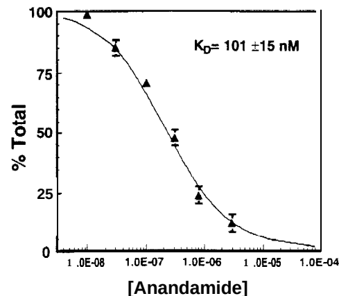
Fig. 9. Anandamide displacement of [ ^3\text{H} ]CP-55,940 binding in the presence of 50 \mu\text{M} PMSF. The data are presented as percent displacement of total binding. K_D = mean \pm S.E. of three experiments.
