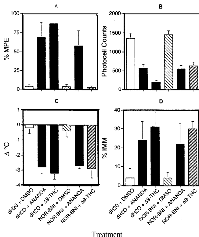
Fig. 8. The effects of 10 \mu\text{g} of i.t. nor -BNI pretreatment followed by 100 \mu\text{g} of i.t. anandamide or 50 \mu\text{g} of \Delta^9 -THC on tail-flick latency (A), motor activity (B), rectal temperature (C) and ring immobility (D). Animals received an i.t. injection of either \text{dH}_2\text{O} or nor -BNI followed 10 min later by a second i.t. injection of either DMSO, \Delta^9 -THC or anandamide. The means ( N = 6 ) \pm S.E. are presented.
