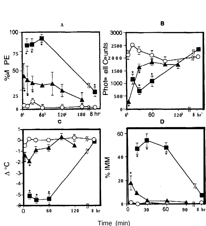
Fig. 4. The time course of effects of i.p. administered vehicle (O), 100 mg/kg of \Delta^9 -THC (■) and 25 mg/kg of anandamide (A) on tail-flick latency (A), motor activity (B), rectal temperature (C) and ring immobility (D). The means \pm S.E. (N = 12) are presented. *Values found to be significantly different ( P < .05 ) than groups receiving vehicle using Scheffe F-test.
