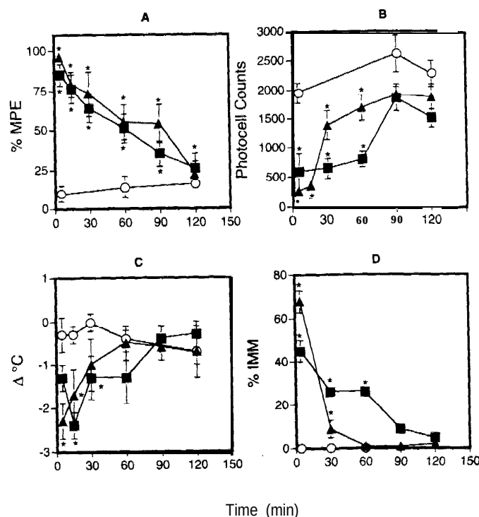
Fig. 2. The time course effects of either 50 mg/kg of anandamide (A), 3 mg/kg of \Delta^9 -THC (B) or vehicle (C) after i.v. administration on tail-flick latency (A), motor activity (B), rectal temperature (C) and ring immobility (D). Animals received a single i.v. injection of either vehicle (1:1:18), \Delta^9 -THC or anandamide and were tested once at the indicated time. The means \pm S.E. ( N = 12 ) are presented. Values found to be significantly different ( P < .05 ) than groups receiving vehicle using Dunnett's t test.
