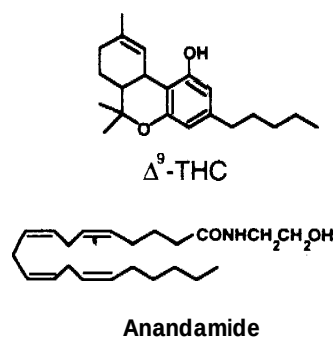
Fig. 1. The structures of \Delta^9 -THC and anandamide.
