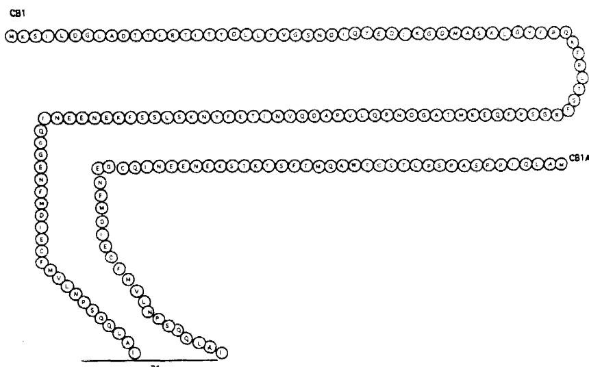
FIG. 2. Proposed amino terminal domains of the human CB1 and CB1A receptors.
