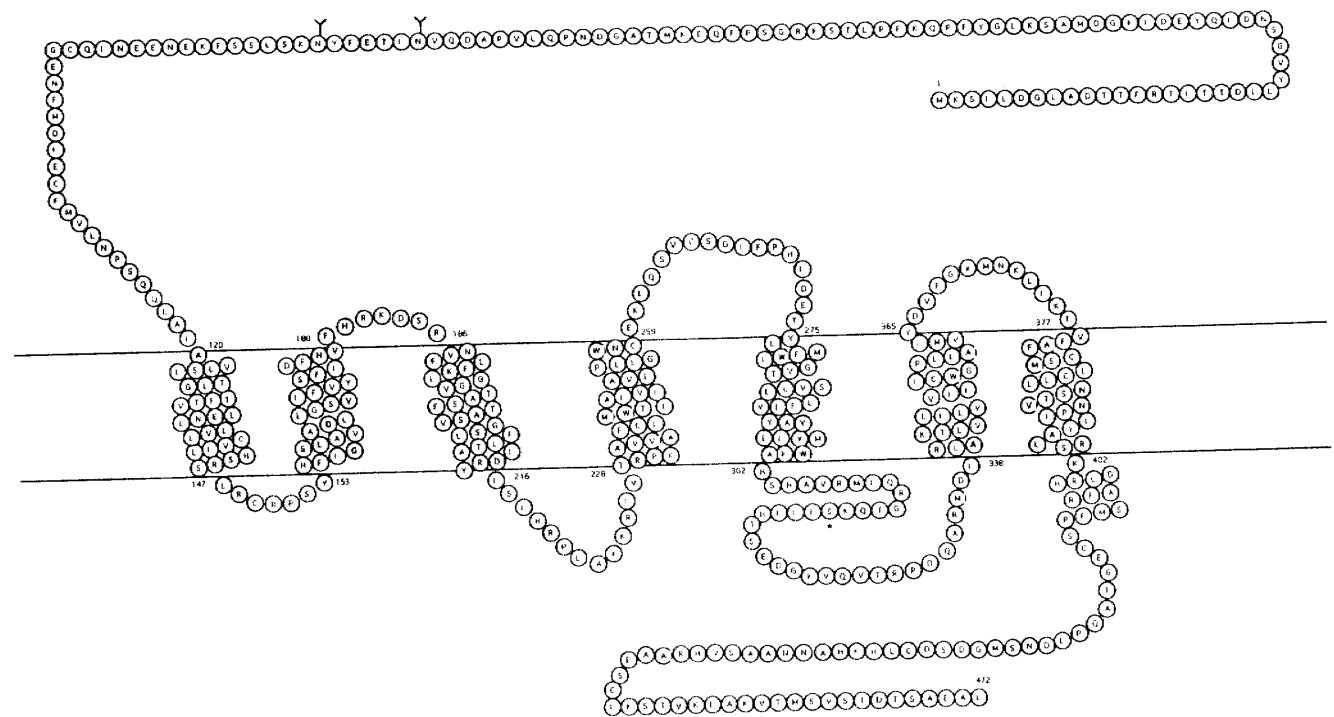
FIG. 1. Proposed membrane topography of the human CB1 cannabinoid receptor. Membrane spanning domains are defined according to hydropathy analysis and determination of helix ends (Bramblett et al. , 1995). Shaded circles indicate amino acids that are conserved between the CB1 and CB2 receptors. Y, potential N-linked glycosylation sites; *, potential phosphorylation sites.
