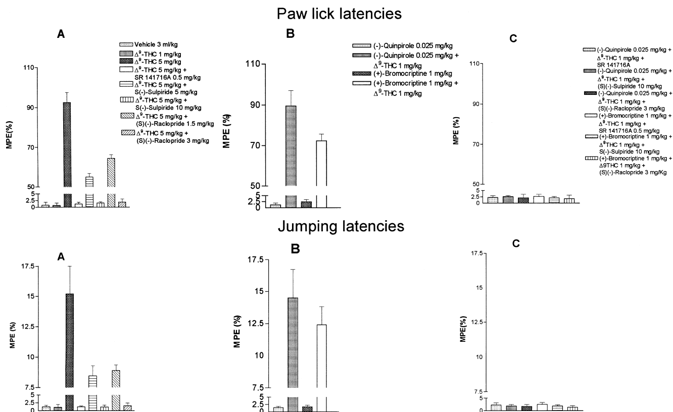
Fig. 1. (A) Blockade of the antinociceptive effects of \Delta^9 -tetrahydrocannabinol by SR 141716A, \text{S}(–) -sulpiride and \text{S}(–) -raclopride in the hot plate test. (B) Potentiation of \Delta^9 -tetrahydrocannabinol effect by (–)-quinpirole and (+)-bromocriptine and (C) reversal by SR 141716A, \text{S}(–) -sulpiride and \text{S}(–) -raclopride. \Delta^9 -tetrahydrocannabinol was given 60 min before the test, while (–)-quinpirole, (+)-bromocriptine, SR 141716A, \text{S}(–) -sulpiride and \text{S}(–) -raclopride were given 20 min before \Delta^9 -tetrahydrocannabinol. Antinociception is expressed as the percent of maximum possible effect (%MPE) in the hot plate test. n = 6 rats per column. All statistical comparisons (Student–Newman–Keuls test) revealed significant differences with P < 0.0001 .
