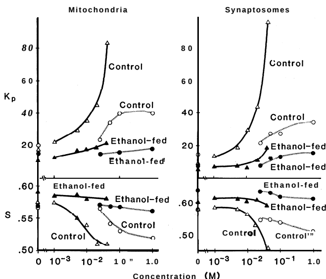
Fig. 1. Effect of ethanol (0, ●) and halothane (Δ, A) on the 5N10 partition coefficient K_p (upper panels) and on the 5-doxyl stearate order parameter S (lower panels) in liver mitochondrial membranes and brain synaptosomal membranes from ethanol-fed rats and their pair-fed controls. EPR spectra were obtained at 35^\circ \pm 0.2^\circ\text{C} with a Varian E-109 spectrophotometer. The nitroxide-decane derivative 5N10 was added to membrane suspensions (10 mg of protein per milliliter) to
