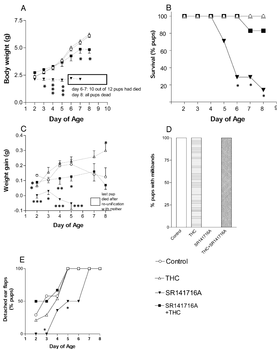
Fig. 1. Week-long administration of antagonist. Mouse pups (Sabra strain) were given two injections (s.c.) each day between days 2 and 8 of life: vehicle (2 ×) (ethanol/cremophor EL/saline = 1:1:18, open circles, n = 10 ), or \Delta^9 -tetrahydrocannabinol (20 mg/kg) and vehicle (open triangles, n = 12 ), or SR141716A (20 mg/kg) and vehicle (closed triangles, n = 12 ), or \Delta^9 -tetrahydrocannabinol and SR141716A (closed squares, n = 12 ). Daily assessments were made of body weights (A); survival rates (B); weight gain upon feeding (C); milkbands in stomachs (D); and ear flap detachment (E); * P < 0.05 ; ** P < 0.01 ; *** P < 0.001 , different from controls.
