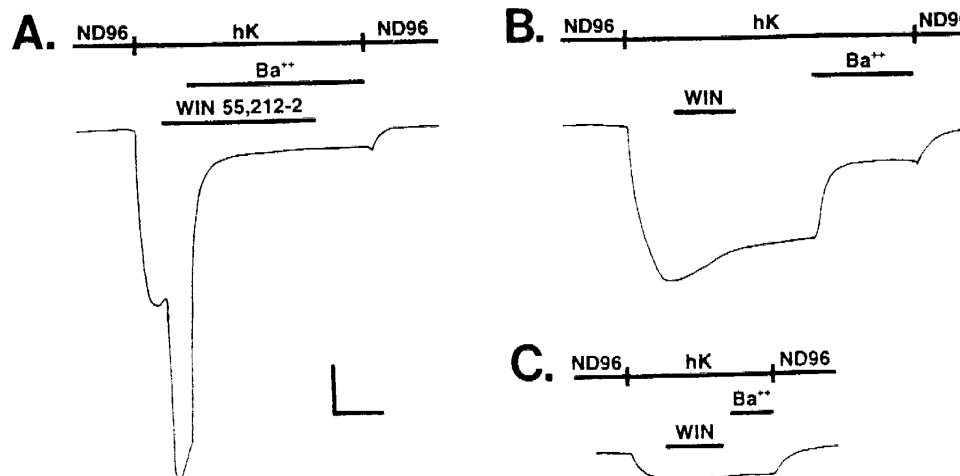
Fig. 1. (A) Inward \text{K}^+ currents evoked in oocytes injected with 10 ng nCANN plus 2 ng GIRK1 cRNA. An inwardly rectifying \text{K}^+ current was induced by exchange of ND96 buffer for high \text{K}^+ (hK) buffer in a representative oocyte voltage clamped at -80 mV. This current was enhanced by introduction of the cannabinoid agonist, WIN 55,212-2 (10 \mu\text{M} ). Introduction of 300 \mu\text{M} \text{Ba}^{2+} blocked the agonist response and left a small, non-GIRK1 mediated component of the inward current response to hK. \text{Ba}^{2+} and hK were washed out simultaneously, resulting in a small inward current tail. (B) Application of the same compounds to an oocyte injected with only GIRK1 channel cRNA (2 ng) resulted in a response to hK but not WIN 55,212-2. The response to hK partially desensitized, which was observed in GIRK1-expressing oocytes in the absence of agonist. (C) An oocyte injected with only nCANN cRNA (10 ng) exhibited no response to WIN 55,212-2 and only a small, \text{Ba}^{2+} -insensitive, non-GIRK1-mediated response to hK. Vertical and horizontal scale bars represent 250 nA and 4 min, respectively, in (A) and 100 nA and 4 min in (B) and (C).
