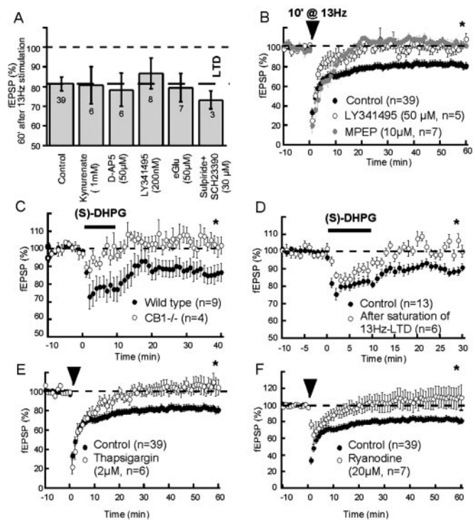
Fig. 4. eCB-LTD is mediated by mGlu5 activation and rise of \text{Ca}^{2+} from intracellular store. (A) Antagonists of ionotropic GluR (kynureneate), NMDAR (D-AP5, 50 \mu\text{M} ), mGlu2/3 [200 nM 2-amino-2-(2-carboxycyclopropan-1-yl)-3-(dibenzopyran-4-yl) propanoic acid and 200 \mu\text{M} (2S), \alpha -ethylglutamic acid], and D1 and D2 receptors (SCH23390 and sulpiride, 30 \mu\text{M} ) do not affect eCB-LTD: fEPSP measured 81.1 \pm 8.8\% ( n = 6 ), 84.0 \pm 3.5\% ( n = 5 ), 73.1 \pm 5.0\% ( n = 3 ), 86.6 \pm 7.9\% ( n = 8 ) and 79.5 \pm 7.2\% ( n = 7 ) of baseline, at 60 min, P = 0.8, 0.2, 0.3, 0.9 , and 0.4 , respectively, vs. control in the absence of antagonists. (B) The mGlu antagonist LY341495 ( 50 \mu\text{M} ) and the highly specific mGlu5 antagonist 2-methyl-6-(phenylethynyl) pyridine ( 10 \mu\text{M} ) suppressed eCB-LTD: fEPSP measured 109.0 \pm 5.2\% ( n = 6 ) and 102.1 \pm 3.0\% ( n = 7 ) of baseline at 60 min, P < 0.05 vs. control without antagonist, respectively. (C) Activation of mGlu5 with (S)-DHPG induced a form of LTD that was absent in \text{CB1}^{-/-} mice: 30 min after (S)-DHPG, fEPSP measured 101.9 \pm 4.9\% of baseline in \text{CB1}^{-/-} ( n = 4 , white dots) and 86.7 \pm 5.2\% in \text{CB1}^{+/+} ( n = 9 , black dots), P < 0.05 . (D) (S)-DHPG-induced-LTD is occluded after saturation of 13-Hz/eCB-LTD: at 30 min fEPSP measured 88.7 \pm 2.1\% ( n = 13 , black dots) and 100.2 \pm 3.6\% ( n = 6 , white dots) of baseline, respectively. (E) Blockade of mGlu5/eCB-LTD after depletion of \text{Ca}^{2+} intracellular pools with the \text{Ca}^{2+} -ATPase inhibitor thapsigargin. (F) Role of ryanodine-sensitive intracellular \text{Ca}^{2+} stores in eCB-LTD. Ryanodine ( 20 \mu\text{M} ) inhibited eCB-LTD: fEPSP measured 109.7 \pm 12.6\% ( n = 7 ) of baseline at 60 min after ryanodine ( 20 \mu\text{M} , 1–2 h) P = 0.03 vs. control without inhibitor.
