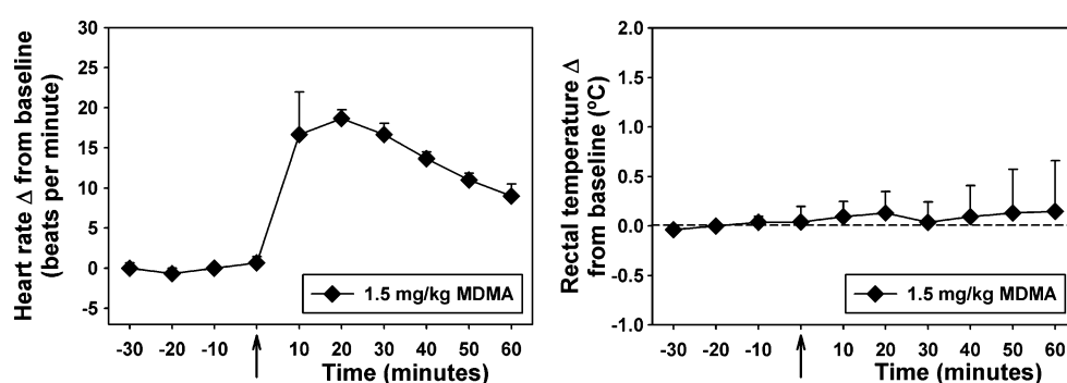
Fig. 5 Effects of 1.5 mg/kg MDMA on heart rate ( left ) and rectal temperature ( right ). Each point represents the mean \pm SEM ( n=3 rhesus monkeys). Abscissae : time (minutes) relative to injection of MDMA. Ordinates : heart rate (beats per minute, left ) or rectal temperature ( ^{\circ} C, right ), reported as a change from baseline
