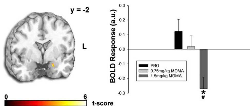
Fig. 3 MDMA effects on amygdala activation. Left Statistical t map overlaid on a canonical brain rendering (MNI coronal y plane=-2) showing greater left amygdala reactivity to angry versus neutral faces in the PBO relative to the MDMA (1.5 mg/kg) condition (PBO > MDMA). Cluster size is 280 mm 3 (35 contiguous voxels). Statistical
