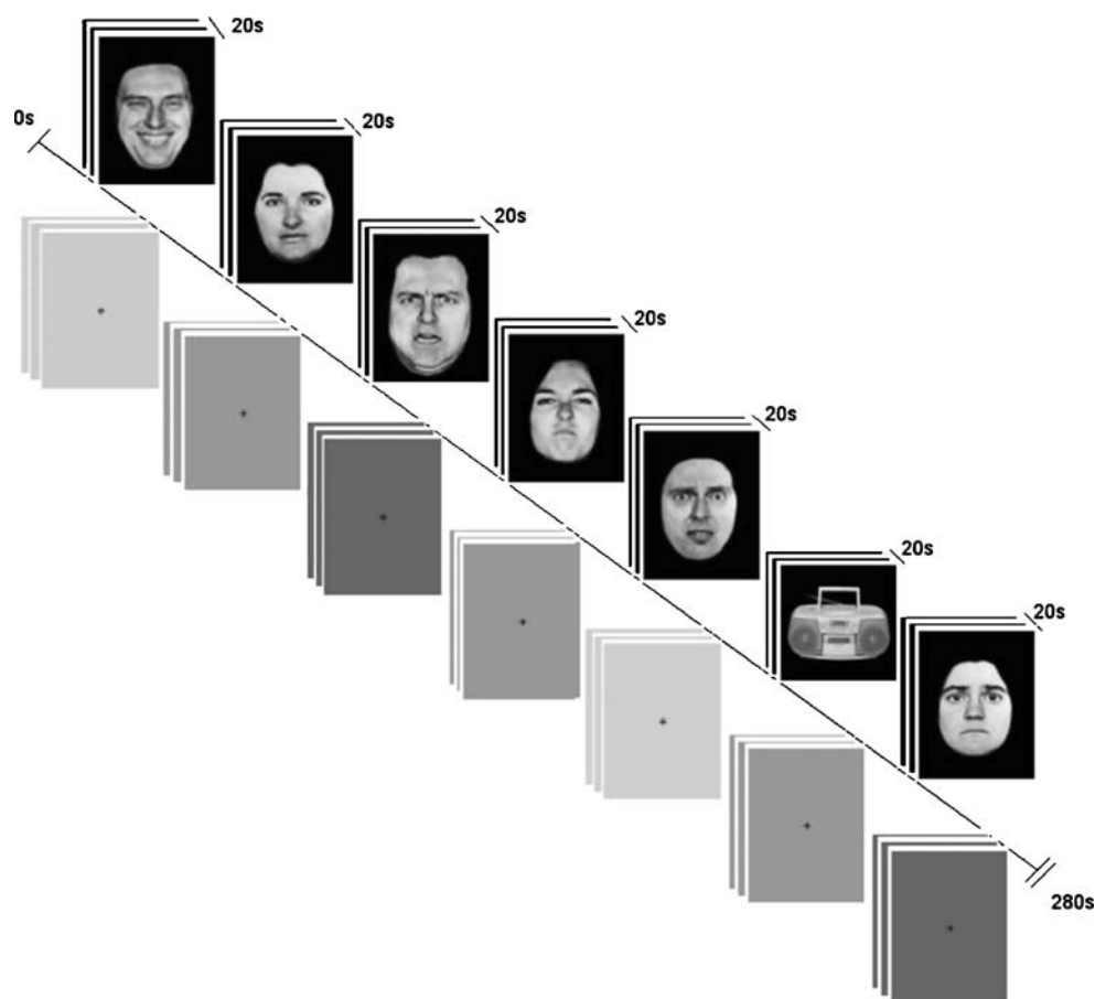
Fig. 1 Schematic of emotional recognition stimuli employed during fMRI
