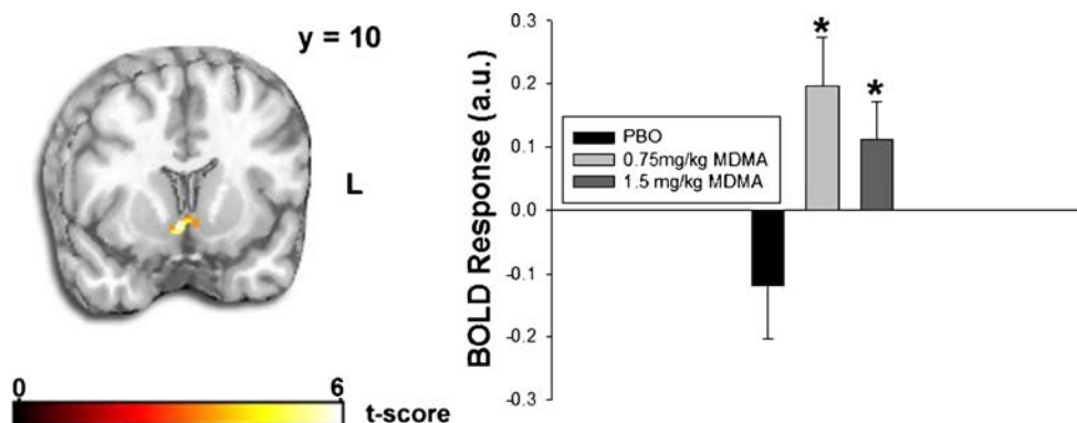
Fig. 4 MDMA effects on ventral striatum activation. Left Statistical t map overlaid on a canonical brain rendering (MNI coronal y plane=10) showing greater ventral striatum reactivity to happy versus neutral faces in the MDMA (0.75 mg/kg) relative to the PBO condition (MDMA > PBO). Cluster size is 1,520 mm 3 (190 contiguous voxels). Statistical
