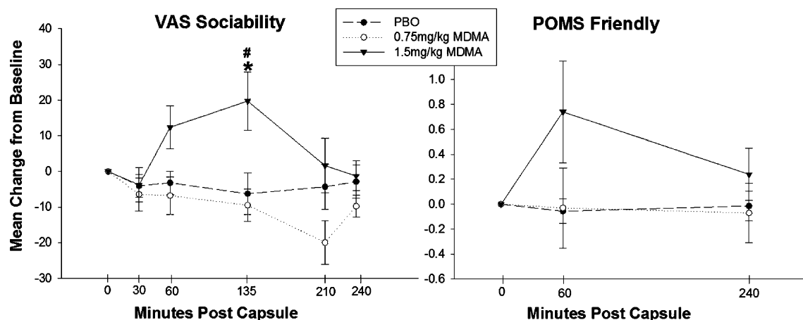
Fig. 2 MDMA effects on self-reported sociability. Left Visual analog scale sociability. Right Profile of mood states friendliness. Data are mean change from pre-drug baseline ( \pm SEM) as a function of minutes
