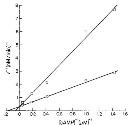
Fig. 5. Lineweaver-Burke plot of cAMP hydrolysis of supernate O and inhibition by 0.8 mM LSD □. cAMP concentration varied from 0.7 to 20.4 \mu M.
