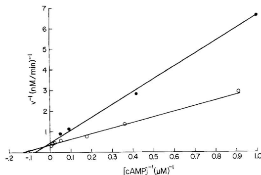
Fig. 1. Lineweaver-Burke plot of cAMP hydrolysis by supernate ○ and particulate ● fractions from F. hepatica . The concentration of cAMP varied from 1.1 to 500 \mu\text{M} for the supernate and from 1.0 to 20.4 \mu\text{M} for the particulate enzyme. The protein concentration of the supernate in the assay was 0.8 mg/ml, and for the particulate it was 1.6 mg/ml. All lines in Lineweaver-Burke plots were drawn by linear regression.
