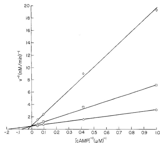
Fig. 4. Lineweaver-Burke plot of cAMP hydrolysis by supernate ○ and inhibition by 20 \mu\text{M} □ and 100 \mu\text{M} ◇ SQ 20009. cAMP concentration varied from 1 to 20.4 \mu\text{M} .
