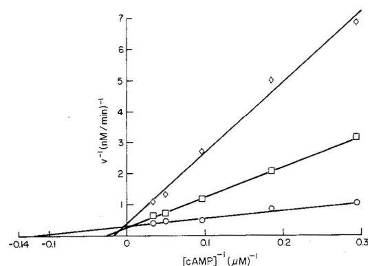
Fig. 2. Lineweaver-Burke plot of cAMP hydrolysis by supernate ○ and inhibition by 100 \mu\text{M} □ and 400 \mu\text{M} ◇ IBMX. cAMP concentration varied from 3.4 to 30.4 \mu\text{M} .
