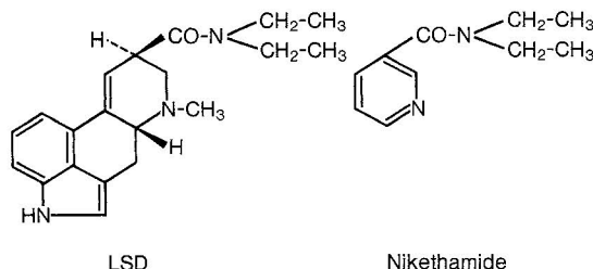
Fig. 1. Structural relationship between LSD and nikethamide
