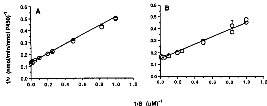
Fig. 3. Lineweaver-Burk plots of the demethylation of MDMA by yeast microsomes expressing CYP2D6. Substrate concentration ranged from 1 to 1000 \mu\text{M} . Panel A, data for (-)-MDMA; panel B, data for (+)-MDMA. The lines are calculated from kinetic constants obtained by fitting the data with a single enzyme site model.
