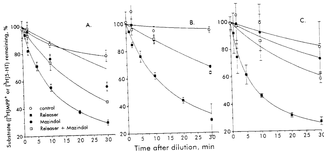
Fig. 3. Inhibition of biogenic amine uptake by amphetamine derivatives in LLC-SERT (A), LLC-NET (B), and LLC-DAT (C) cells. Uptake rates for [^3\text{H}]\text{5-HT} (A) and [^3\text{H}]\text{MPP}^+ (B and C) were measured in 4-min incubations at room temperature, with the indicated concentrations of the following compounds: amphetamine (AMPH), MDMA, METH, PCA, methylphenidate (MePh), and MMAI.
