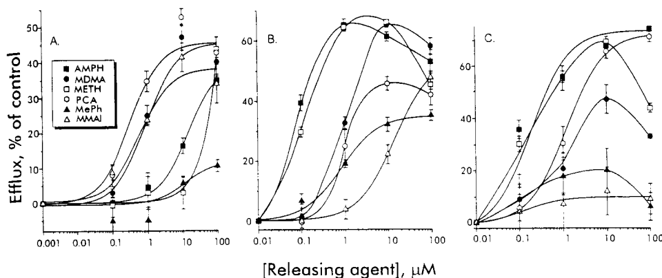
Fig. 5. Concentration dependence for biogenic amine efflux from LLC-SERT (A), LLC-NET (B), and LLC-DAT (C) cells. Cells were allowed to accumulate [ ^3 H]-HT (A) or [ ^3 H]MPP ^+ (B and C) for 30 min. The external substrate was removed by dilution with fresh medium containing the indicated concentration of the following releasing agents: amphetamine (AMPH), MDMA, METH, PCA, methylphenidate (MePh), and MMAI. After 30 min at room temperature, the cells were washed and counted to determine remaining internal radiolabel. Efflux was calculated as the percentage of radiolabel lost from the cells, relative to the control (dilution into medium containing no releasing agent).
