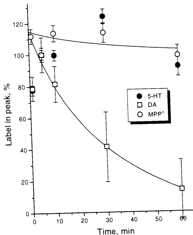
Fig. 2. Degradation of DA, 5-HT, and MPP^+ by transfected LLC-PK 1 cells. Stability of substrates in transfected cells was determined as follows. Cells were incubated with radiolabeled transport substrates under normal transport assay conditions. [^3H]DA was incubated with LLC-DAT cells ( \square ), [^3H]MPP^+ with LLC-NET cells ( \circ ), and [^3H]5-HT with LLC-SERT cells ( \bullet ). After the time indicated, a sample of the supernatant medium was taken for analysis by HPLC, as described in Experimental Procedures. The fraction of radiolabel coeluting with authentic substrate is plotted as a percentage of the total, with each time course curve normalized to 100% at 5 min to allow better comparison between substrates.
