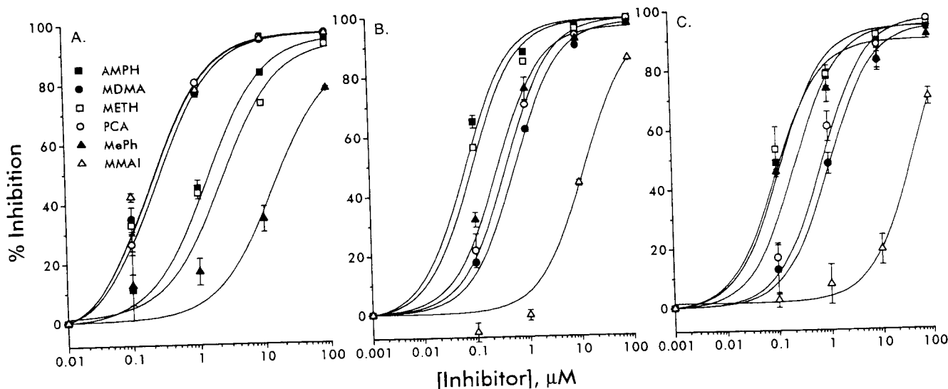
Fig. 3. Inhibition of biogenic amine uptake by amphetamine derivatives in LLC-SERT (A), LLC-NET (B), and LLC-DAT (C) cells. Uptake rates for [^3\text{H}]\text{5-HT} (A) and [^3\text{H}]\text{MPP}^+ (B and C) were measured in 4-min incubations at room temperature, with the indicated concentrations of the following compounds: amphetamine (AMPH), MDMA, METH, PCA, methylphenidate (MePh), and MMAI.
