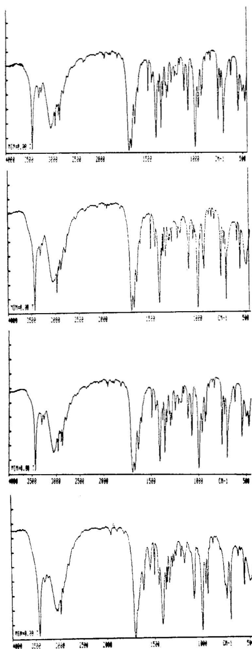
FIG. 11—IR. Top trace: trans -(4 R , 5 R )-4-methylaminorex; second trace: cis -(4 S , 5 R )-4-methylaminorex; third trace: racemic-dl- trans -4-methylaminorex; bottom trace: racemic-dl- cis -4-methylaminorex.
