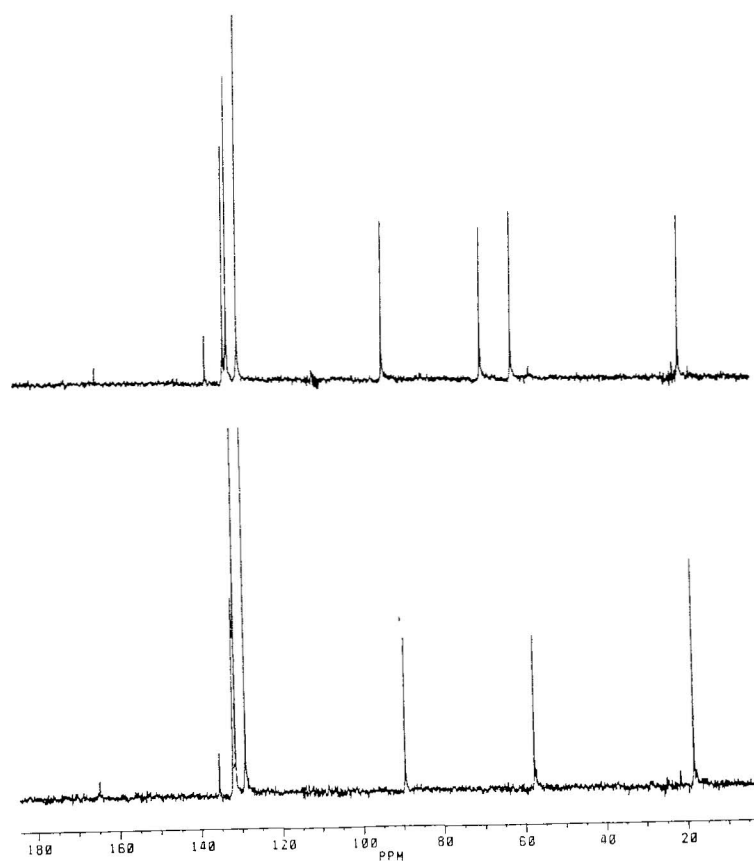
FIG. 10— ^{13}\text{C} -NMR, 20 000 scans (auto-recur). Top trace: trans -(4 R , 5 R )-4-methylaminorex hydrochloride (additional peak at \delta = 66.4 ppm is internal dioxane standard); bottom trace: cis -(4 S , 5 R )-4-methylaminorex hydrochloride. For conditions, see Table 4.
