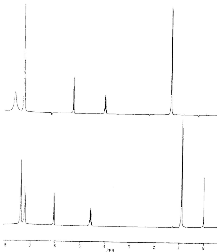
FIG. 9— ^1\text{H} -NMR, 16 scans. Top trace: trans-(4R, 5R)-4-methylaminorex hydrochloride; bottom trace: cis-(4S, 5R)-4-methylaminorex hydrochloride ( -\text{NH}_3^+ off-scale at \delta = 9.12 ppm). For conditions, see Table 4.
