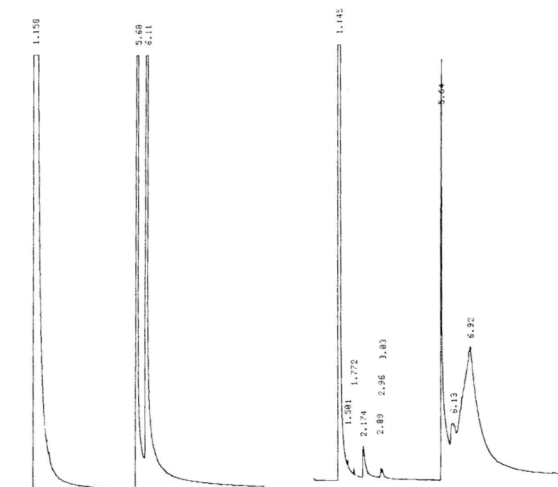
FIG. 6—Left-hand trace: capillary GC of cis -(4 S , 5 R )- and trans -(4 R , 5 R )-4-methylaminorex 1:1 (first eluting compound is the trans isomer). Right-hand trace: trans -(4 R , 5 R )-4-methylaminorex hydrochloride (the cis isomer exhibits similar decomposition). For conditions, see Table 1.
