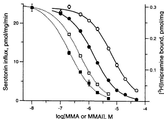
Fig. 1. Inhibition of platelet plasma membrane serotonin transport and imipramine binding. Rates of serotonin influx (---) were measured in 20-sec incubations as described in Experimental Procedures, using 0.1 \mu M [ ^3 H]serotonin in the presence of the indicated concentrations of MMA (■) or MMAI (□). Uptake values due to nonspecific processes, measured in the presence of 1 \mu M imipramine, were subtracted from each measurement. Half-maximal inhibition of transport occurred at 205 \pm 15 nM MMA and 452 \pm 18 nM MMAI. Imipramine binding (—) was measured as described in Experimental Procedures, using 1 nM [ ^3 H]imipramine in the presence of the indicated concentrations of MMA (●) or MMAI (○). Nonspecific binding, measured in the presence of 100 \mu M serotonin, was subtracted from each measurement. Half-maximal inhibition of binding occurred at 1.4 \pm 0.45 \mu M MMA and 6.54 \pm 0.65 \mu M MMAI. Each point represents the average of triplicate determinations. Error bars represent the standard deviation and are plotted only where they exceeded the size of the symbol.
