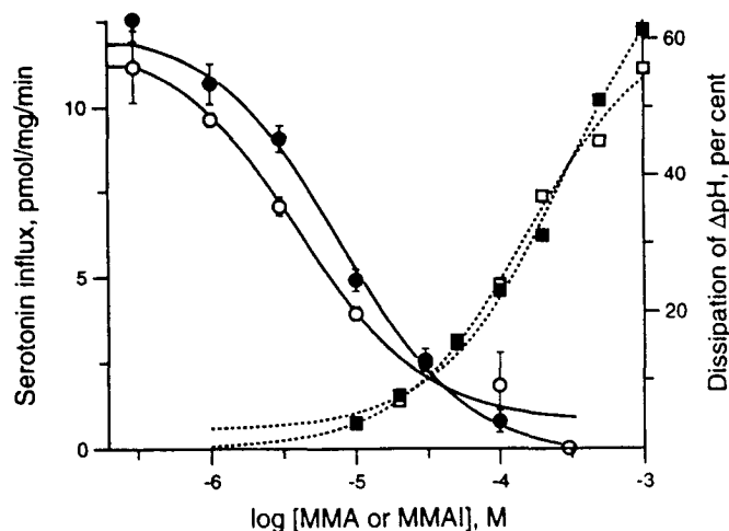
Fig. 3. Inhibition of serotonin transport and dissipation of \Delta pH in chromaffin granule membrane vesicles by MMA and MMAI. For transport measurements (circles), MMA (closed symbols) or MMAI (open symbols) was added at the indicated concentration to the serotonin transport reaction, performed as described in Experimental Procedures. The control rate of transport was 28 pmol/mg/min in the absence of additions. The serotonin concentration used, 0.1 \mu M, is below the K_m (4.3 \mu M) (29). Half-maximal inhibition of transport required 7.7 \pm 1.0 \mu M MMA or 3.9 \pm 0.63 \mu M MMAI. For \Delta pH dissipation measurements (squares), reversal of acridine orange quenching was determined at various MMA and MMAI concentrations as described in Experimental Procedures. The dissipation of \Delta pH is presented relative to the effect of 20 mM \text{NH}_4\text{Cl} . Half-maximal dissipation of \Delta pH required approximately 0.29 \pm 0.05 mM MMA and 0.16 \pm 0.3 mM MMAI. Each point represents the average of triplicate determinations for the transport measurements and duplicates for the \Delta pH measurements. Error bars represent the standard deviation and are plotted only where they exceeded the size of the symbol.
