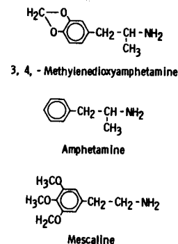
FIG. 1—Chemical structures of 3,4-methylenedioxyamphetamine, amphetamine, and mescaline.
