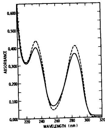
FIG. 2—Ultraviolet spectra in 0.5 N sulfuric acid of 15 µg/ml of standard MDA (solid line) and spot eluted from TLC (broken line).
