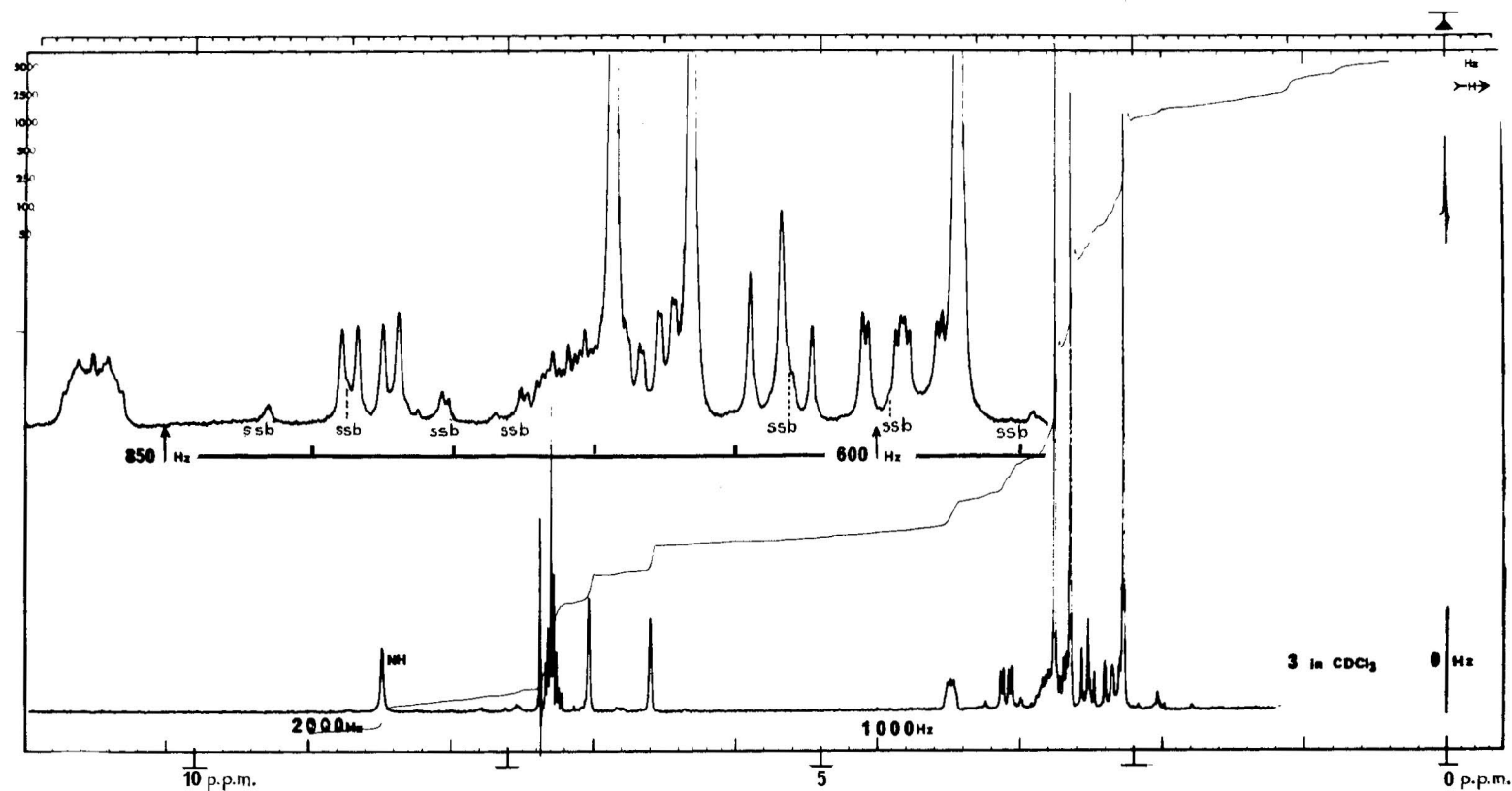
FIG. 1. 220 MHz spectrum of 3 in \text{CDCl}_3 solution. Lower trace: sweep width 2500 Hz. Insert: 5 \times expansion of signals from \delta 2.59–3.98 p.p.m., spinning side-bands are indicated by s.s.b.
