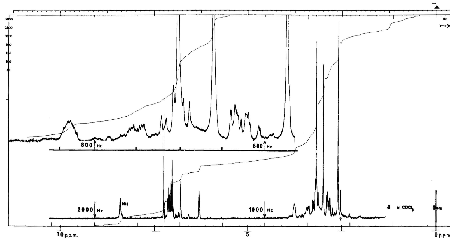
FIG. 3. 220 MHz spectrum of 4 in \text{CDCl}_3 solution. Lower trace: sweep width 2500 Hz. Insert: 5 \times expansion of signals from \delta 2.59–3.78 p.p.m.
