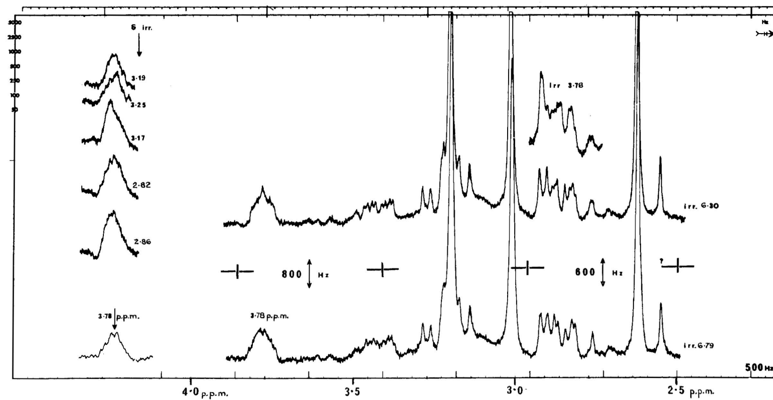
FIG. 4. 220 MHz spectrum of 4 in CDCl 3 solution, sweep width 500 Hz, signals from \delta 2.59–3.78 p.p.m. Upper main trace with irradiation at \delta 6.30 p.p.m.; lower trace with irradiation at \delta 6.79 p.p.m. Inserts as in Fig. 2.
