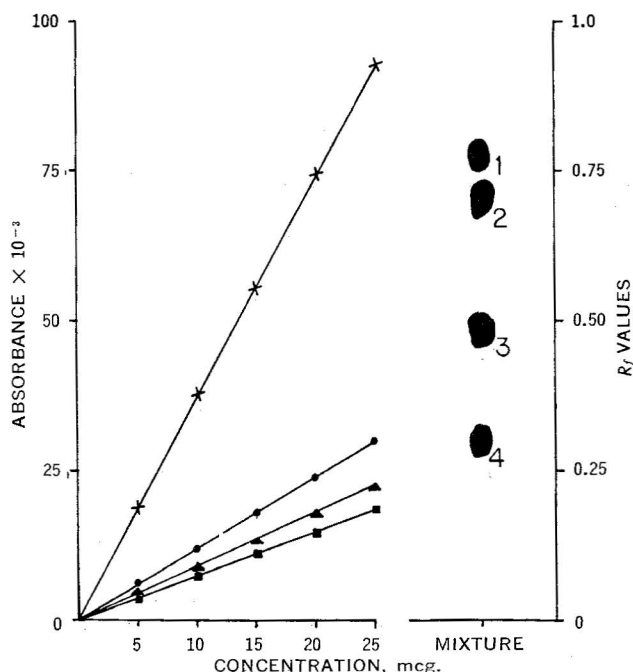
Figure 1 —UV absorption-concentration relationship (left) and R_f values (right) of the following compounds: 1, \times , phenobarbital; 2, \circ , methadone hydrochloride; 3, \Delta , dextroamphetamine; and 4, \blacksquare , ephedrine hydrochloride.
