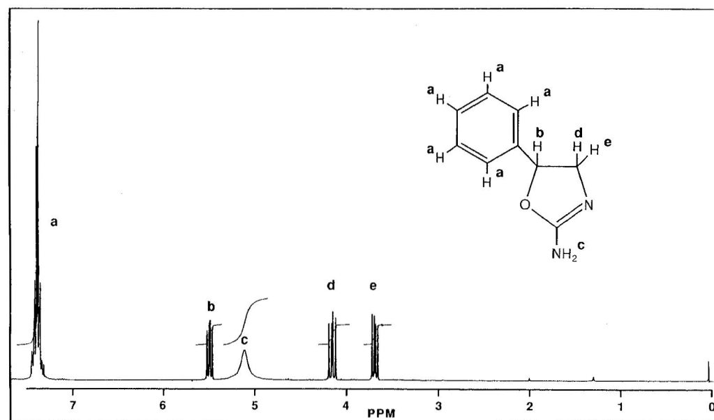
FIG. 2—Proton (300-mHz) NMR spectrum for aminorex with interpretation.
