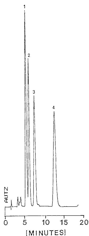
Figure 3. Liquid chromatographic separation of the isomeric (3,4-methylenedioxyphenyl)amines. Peaks: 1 = N,N-dimethyl-1-(3,4-methylenedioxyphenyl), 2 = N-ethyl-1-(3,4-methylenedioxyphenyl), 3 = N-methyl-(3,4-methylenedioxyphenyl)-2-propanamine (MDMA), 4 = 1-(3,4-methylenedioxyphenyl)-2-butanamine. u-Bondapak C 18 column and a mobile phase of pH 3 phosphate buffer, methanol, acetonitrile and triethylamine (600:100:25:1).
