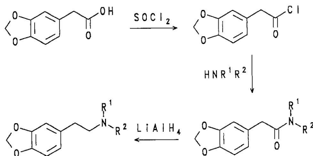
Scheme 1. Synthesis of N-ethyl- and N,N-dimethyl-1-(3,4-methylenedioxyphenyl)-2-ethanamines.
