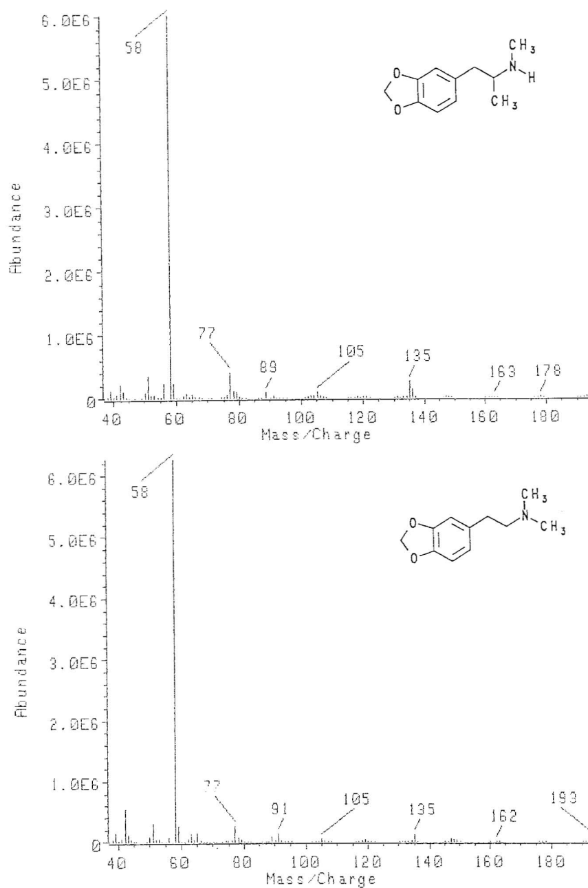
Figure 1. Mass spectra for the four isomeric 1-(3,4-methylenedioxyphenyl)amines.
