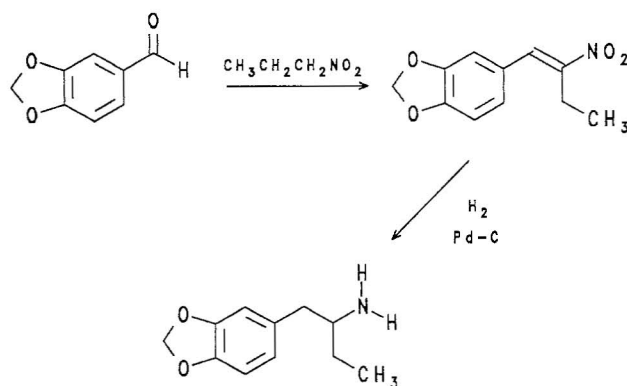
Scheme 2. Synthesis of 1-(3,4-methylenedioxyphenyl)-2-butanamine.
