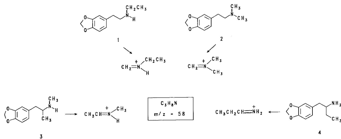
Scheme 3. Electron impact fragmentation pathway for the isomeric 1-(3,4-methylenedioxyphenyl)amines.
