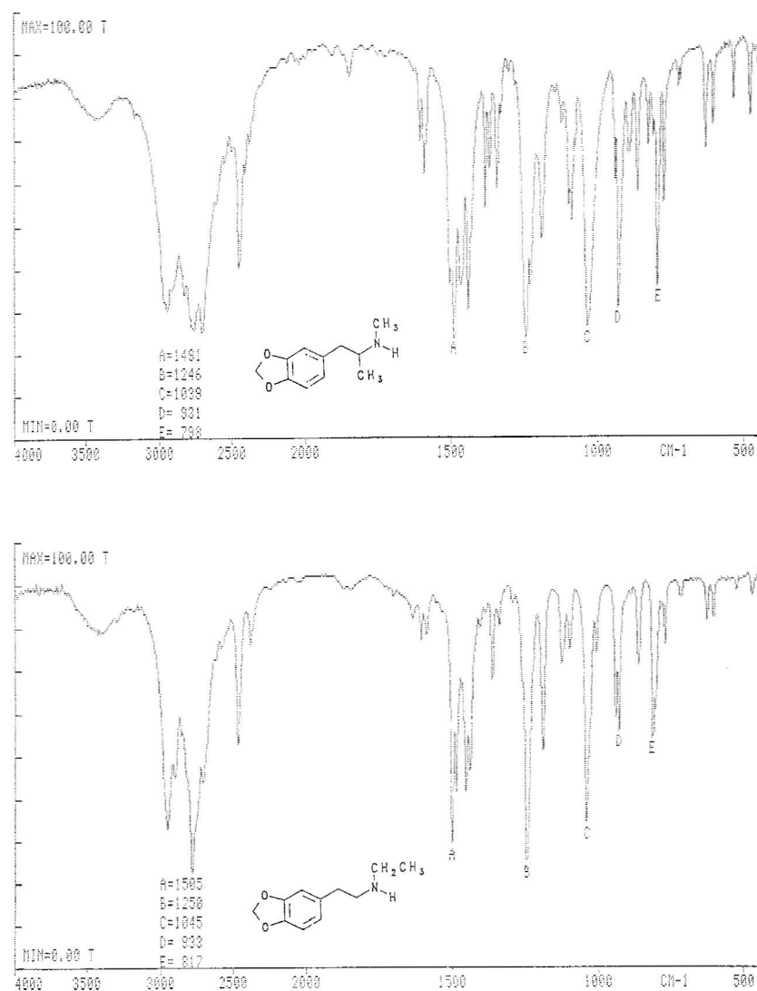
Figure 2. FT-IR spectra for the hydrochloride salts of MDMA (A) and N-ethyl-1-(3,4-methylenedioxyphenyl)-2-ethanamine (B).
