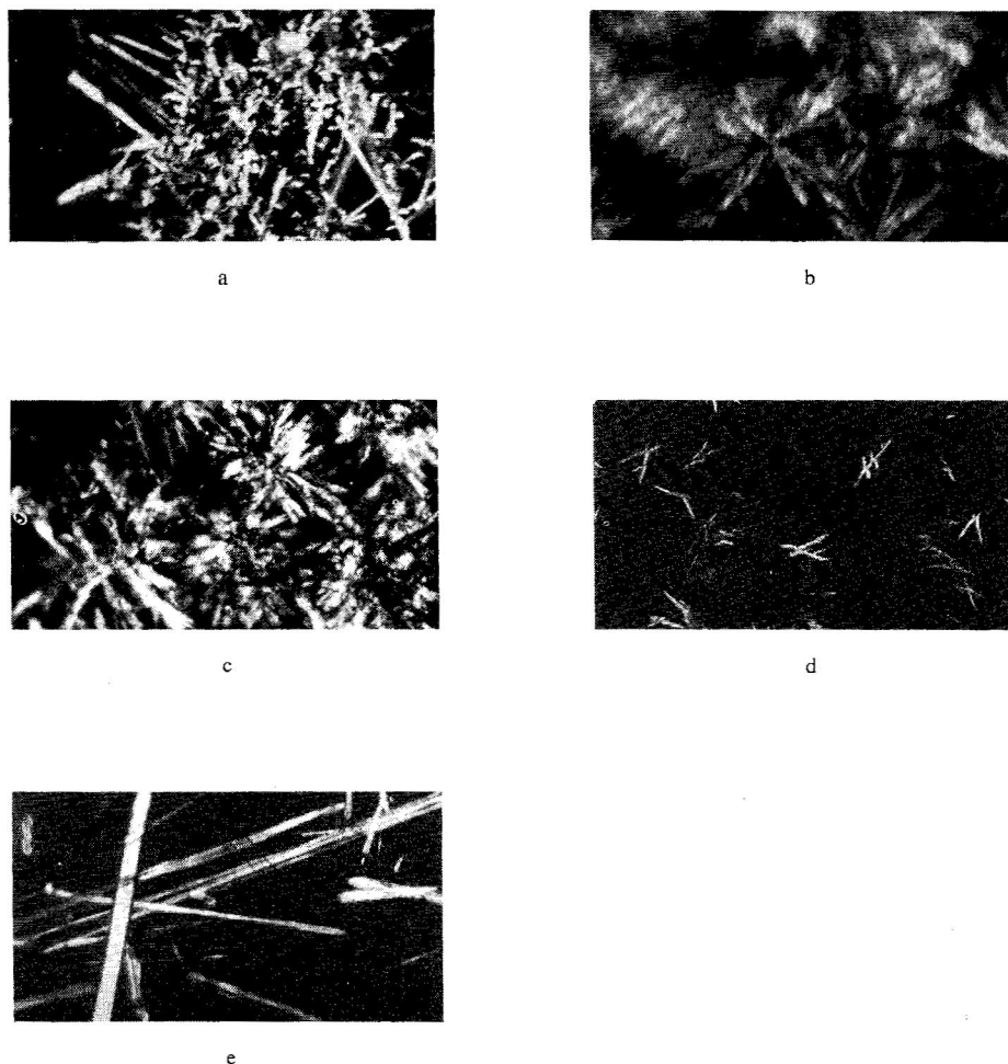
FIG. 1—Most identifiable crystal formations for (a) 3,4-methylenedioxyamphetamine, (b) 3,4-methylenedioxymethamphetamine, (c) 3,4-methylenedioxy-N-ethylamphetamine, (d) mescaline, and (e) 2,5-dimethoxy-4-ethylamphetamine.
