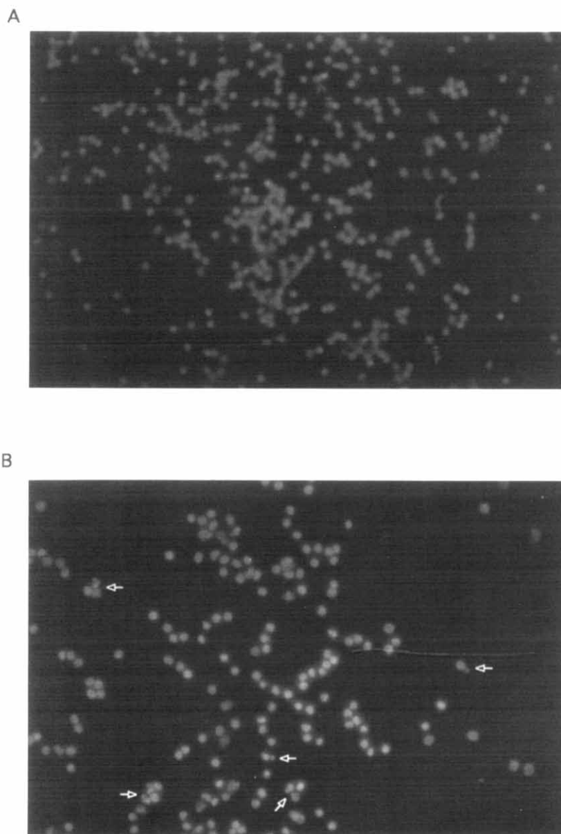
Fig. 4. Anandamide induces DNA fragmentation. PBMC were treated with cannabinoids for 21 h. The cells were collected, fixed and stained with DAPI. Photomicrographs (20 \times ) of representative fields are shown. Bright cells are stained with DAPI and are apoptotic. Apoptotic bodies are indicated by arrows. (A) Untreated cells. (B) 7.5 \times 10^{-5} M anandamide-treated cells.
