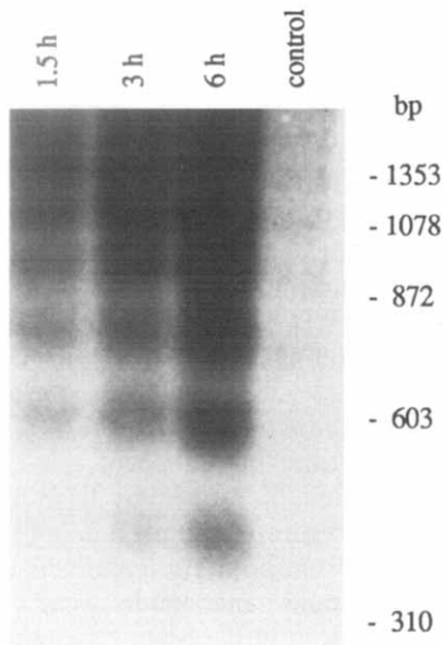
Fig. 5. High concentrations of anandamide cause apoptosis. PBMC were incubated with 7.5 \times 10^{-5} M anandamide for the indicated time intervals. DNA was extracted and analyzed by Southern blotting.
