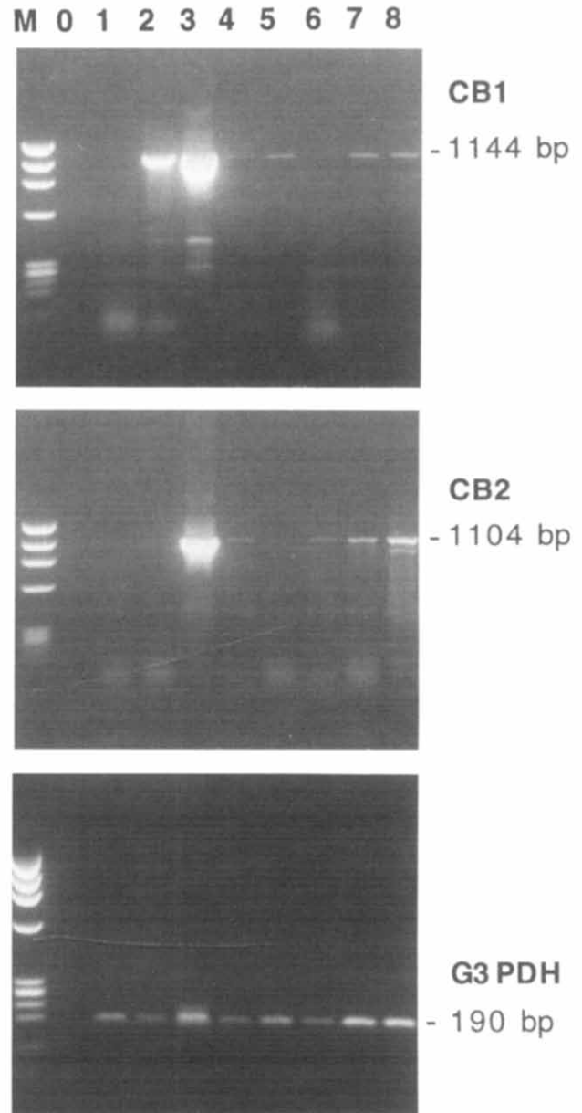
Fig. 7. Donor variability in cannabinoid receptor mRNA expression. PBMC were isolated from eight different donors (nos. 1–8), RNA was extracted and analyzed for CB1 and CB2 expression by RT-PCR. To document similar amounts of RNA and cDNA, the samples were also analyzed for G3PDH. 0 represents the negative PCR control (no template).
