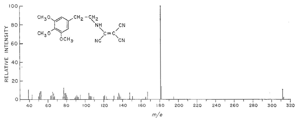
Fig. 2. The 70-V mass spectrum of N-tricyanovinylmescaline (XX) at 180°.
