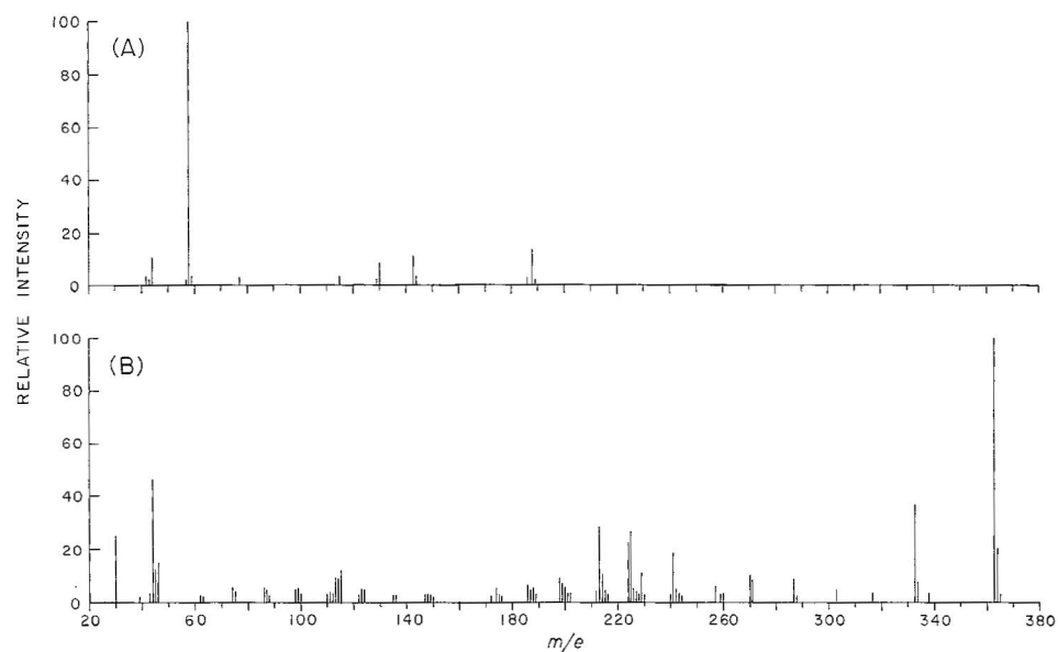
Fig. 1. The 70-V mass spectra of the N ω , N ω -dimethyltryptamine-CNTNF complex at different sample temperatures: (A) spectrum at 121° ( N ω , N ω -dimethyltryptamine) and (B) spectrum at 198° (CNTNF).
